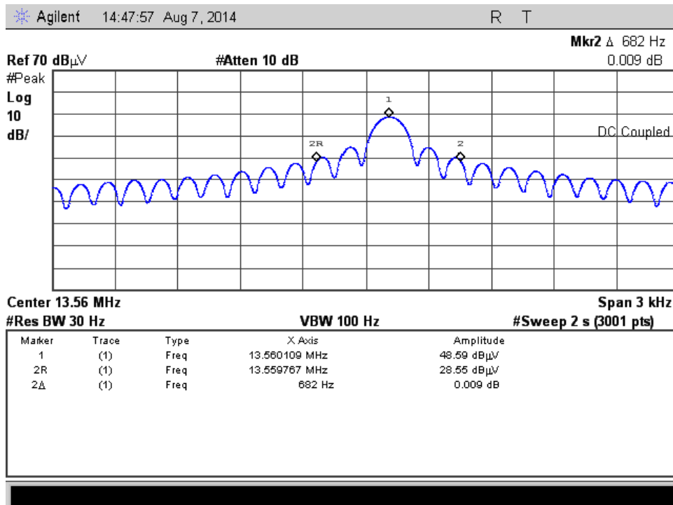
Figure 7.2.2-1: 20dB BW
