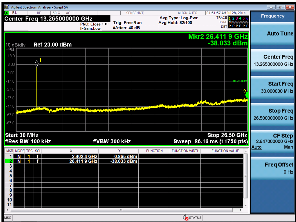
(Plot 4.7.3 A2: Channel 00: 2402MHz @8DPSK)
