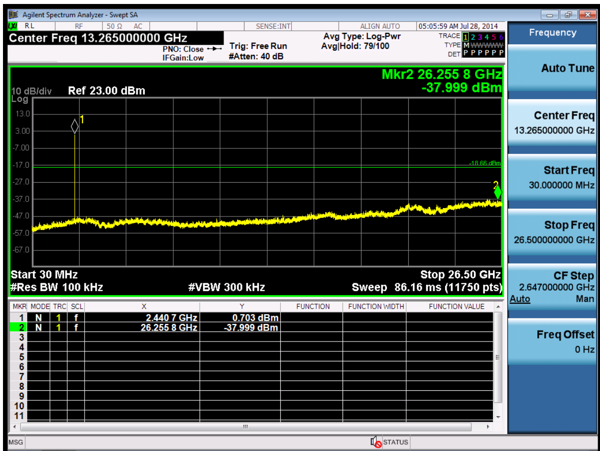
(Plot 4.7.3 B2: Channel 39: 2441MHz @8DPSK)
