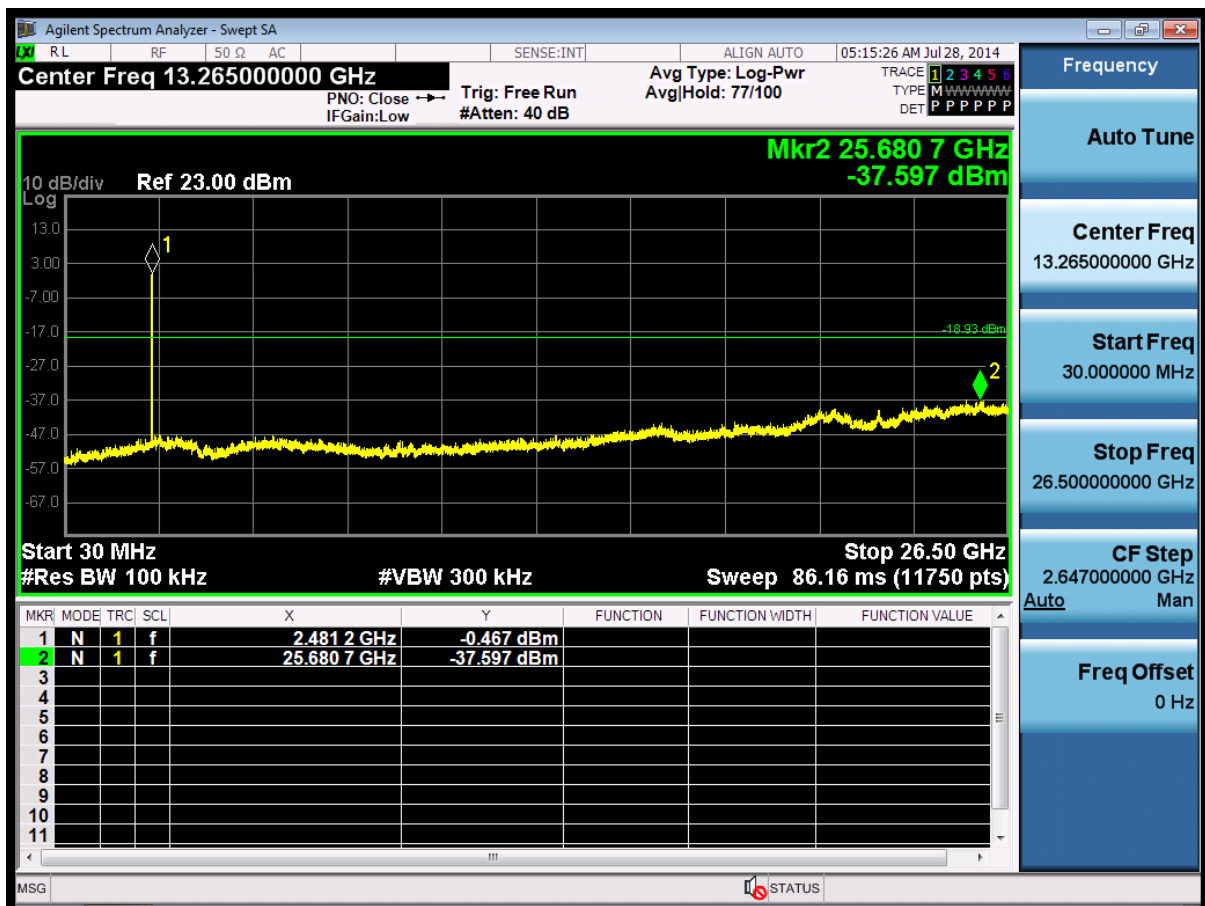
(Plot 4.7.3 C2: Channel 78: 2480MHz @8DPSK)
