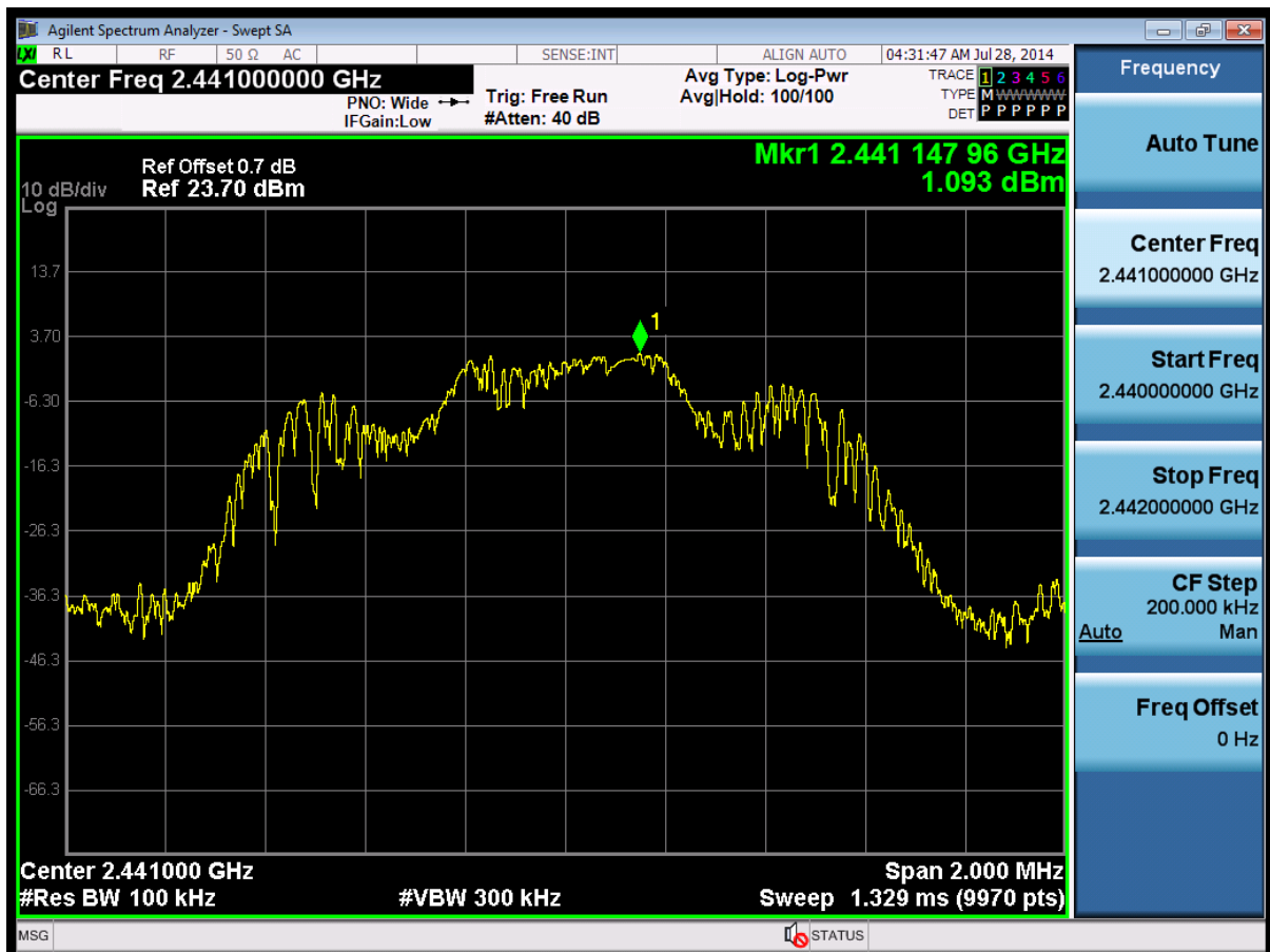
(Plot 4.7.2 B1: Channel 39: 2441MHz @ \pi/4 DQPSK)
