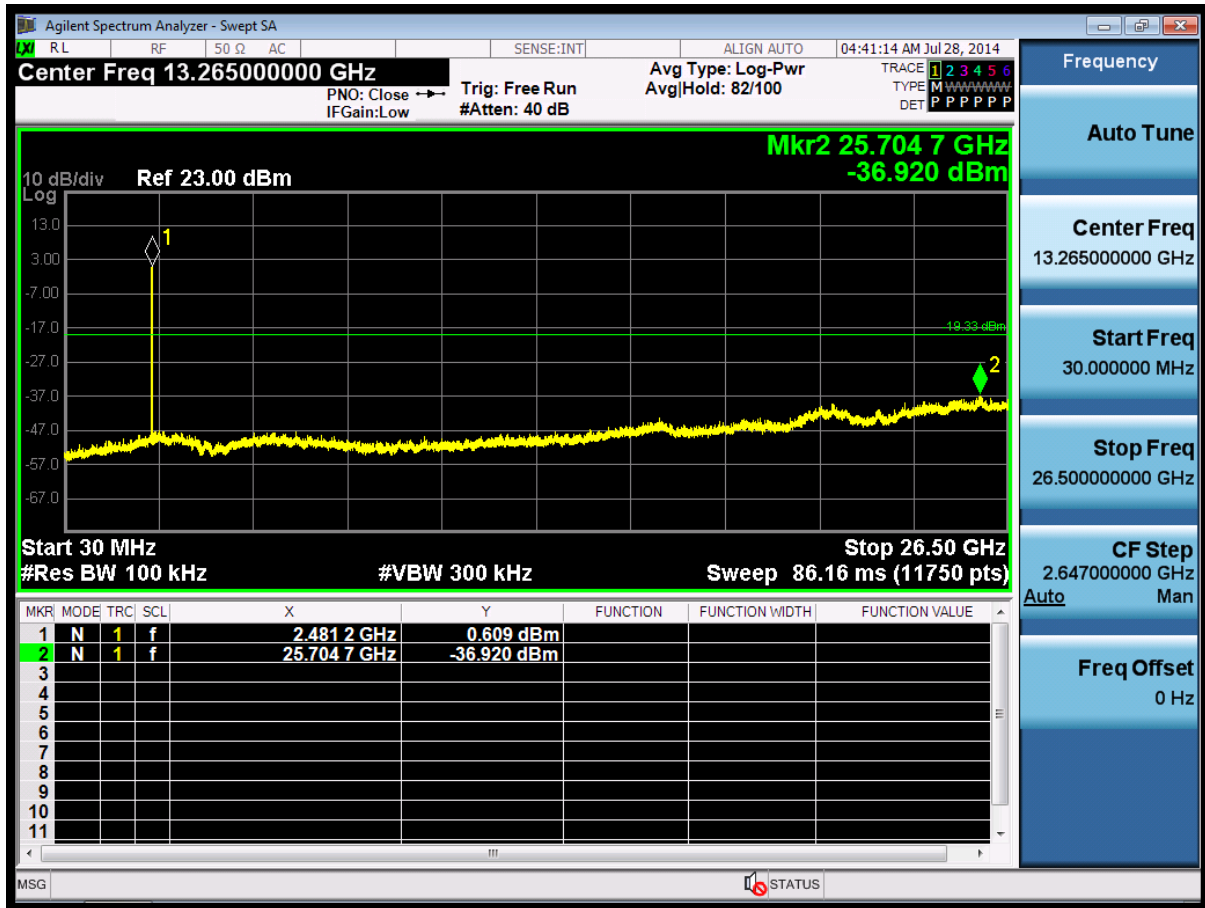
(Plot 4.7.2 C2: Channel 78: 2480MHz @ \pi/4 DQPSK)
