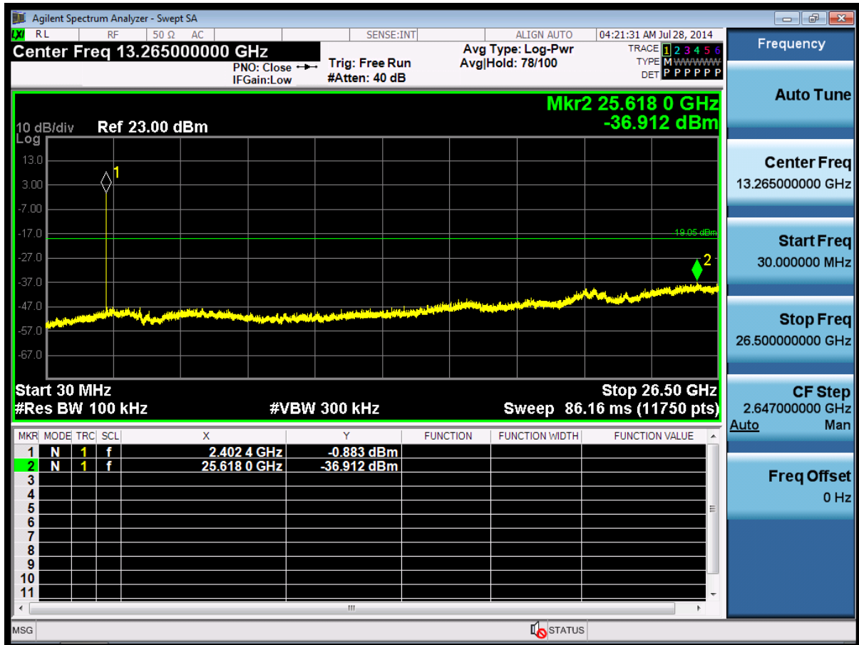
(Plot 4.7.2 A2: Channel 00: 2402MHz @ \pi/4 DQPSK)
