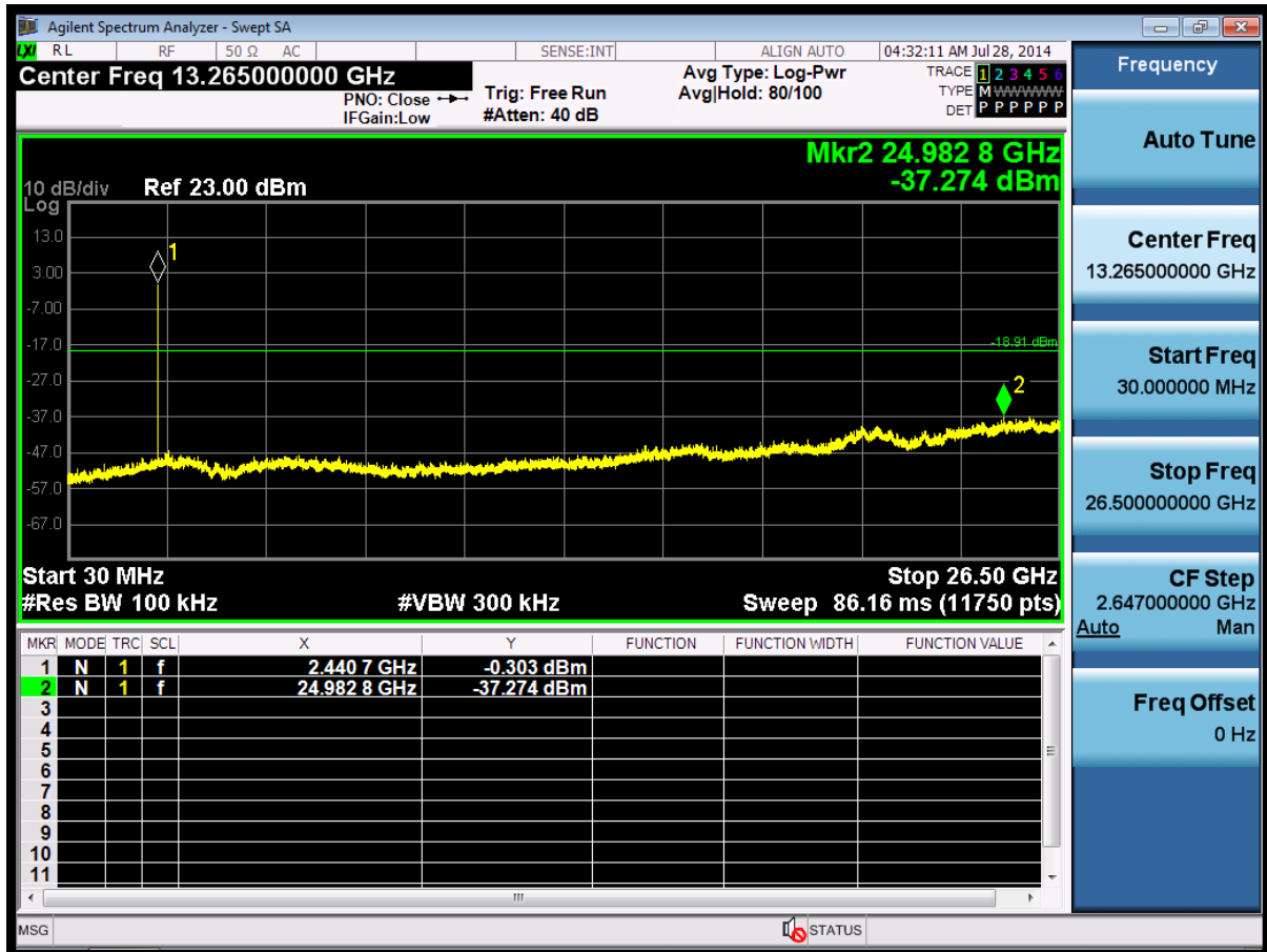
(Plot 4.7.2 B2: Channel 39: 2441MHz @ \pi/4 DQPSK)
