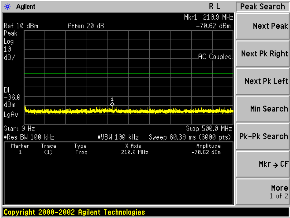
TEST PLOT OF OUT OF BAND EMISSIONS OF \pi/4 -DQPSK MODULATION IN MIDDLE CHANNEL
