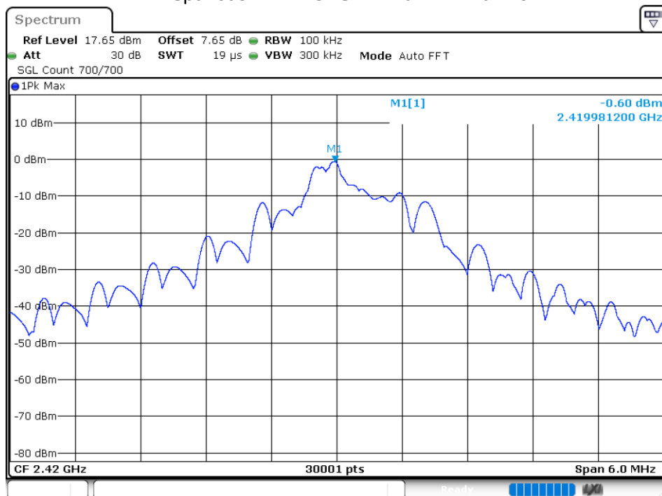
Tx. Spurious NVNT GFSK 2420MHz Ant1 Ref
