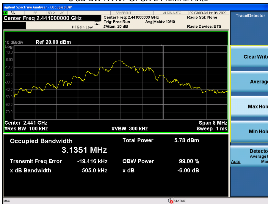
-6 dB BW NVNT GFSK 2441MHz Ant1
