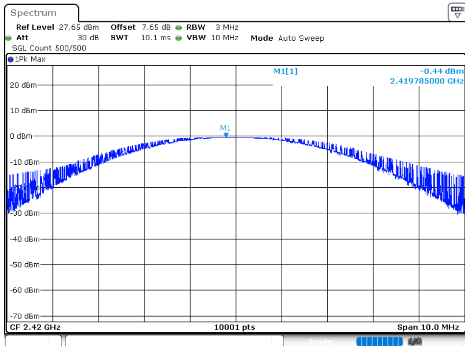
Power NVNT GFSK 2420MHz Ant1
