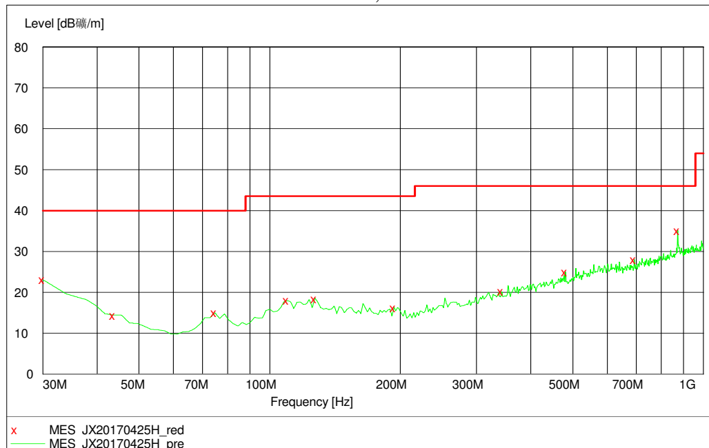
30MHz~1GHz, Horizontal
