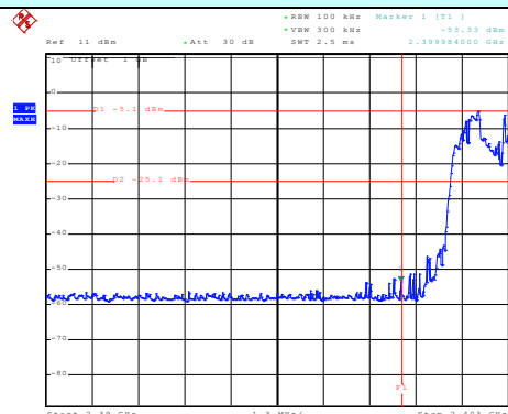
Hopping mode
