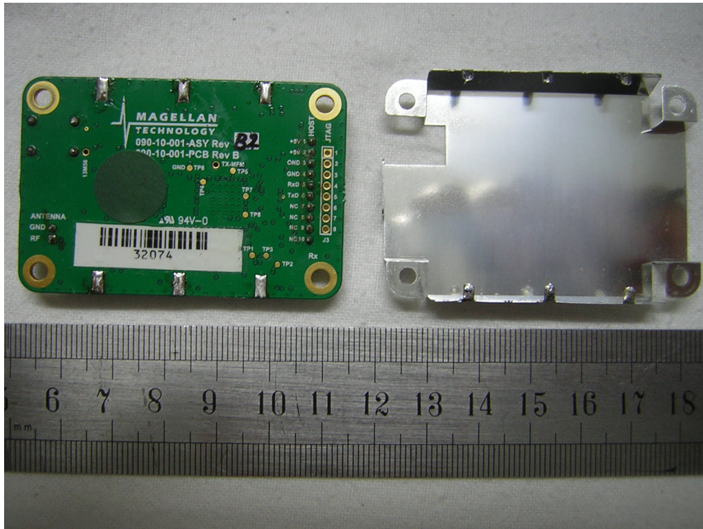
RF Module inside – cover removed
