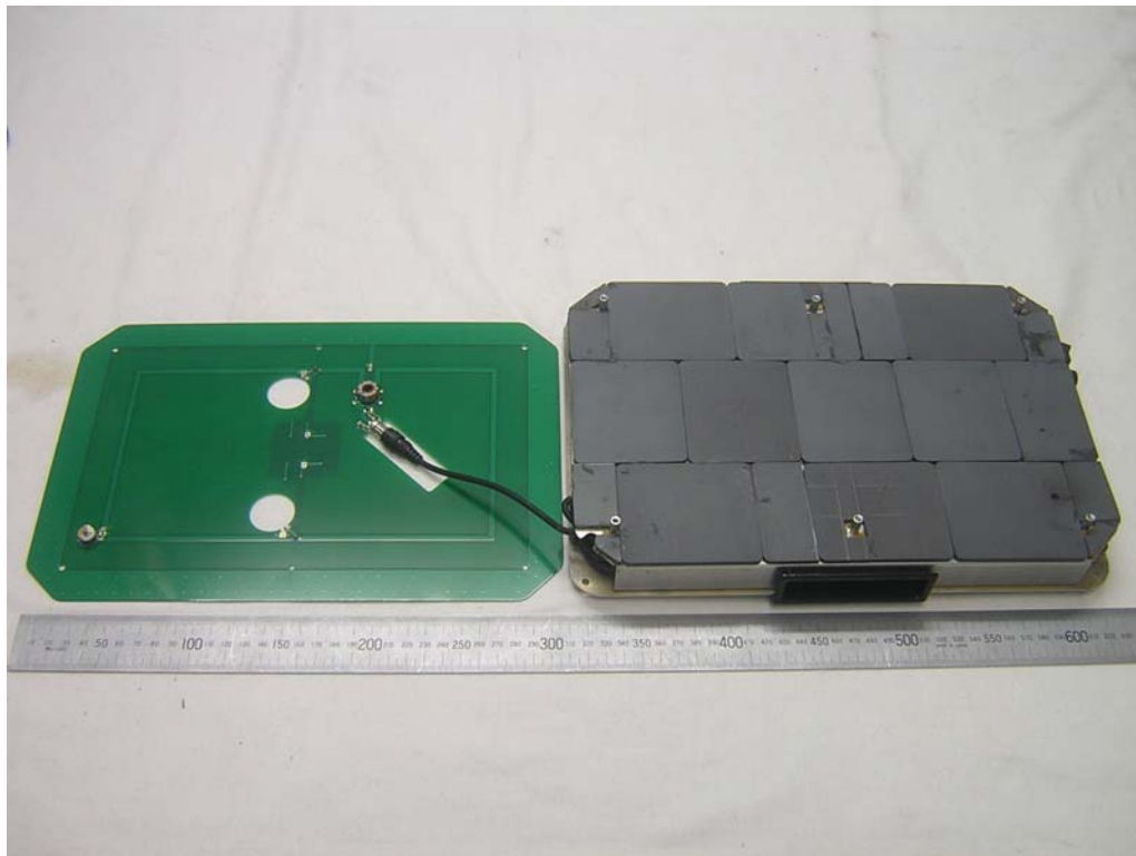
EUT Antenna with Ferrites
