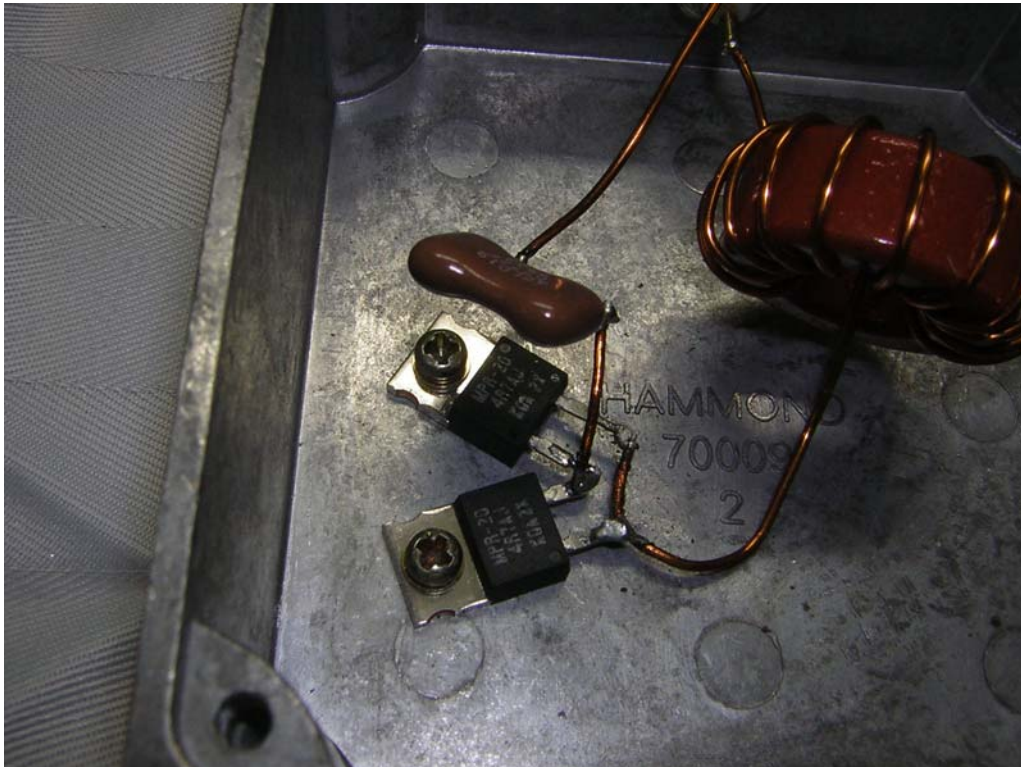
Internal of 50 \Omega Termination Box
