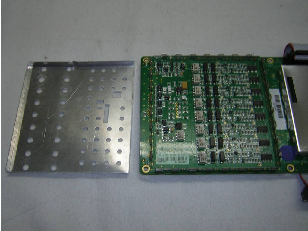
PCB 3
