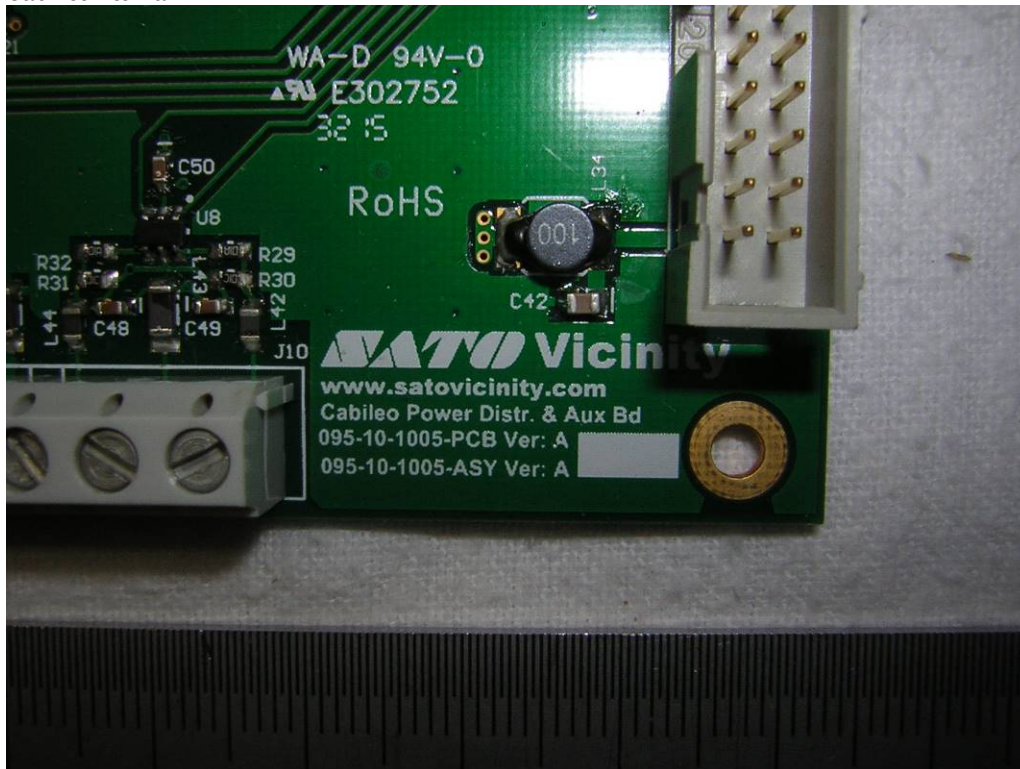
Cabinet Internal
