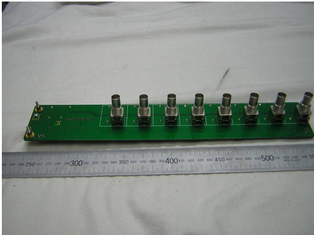
PCB Antenna Interface
