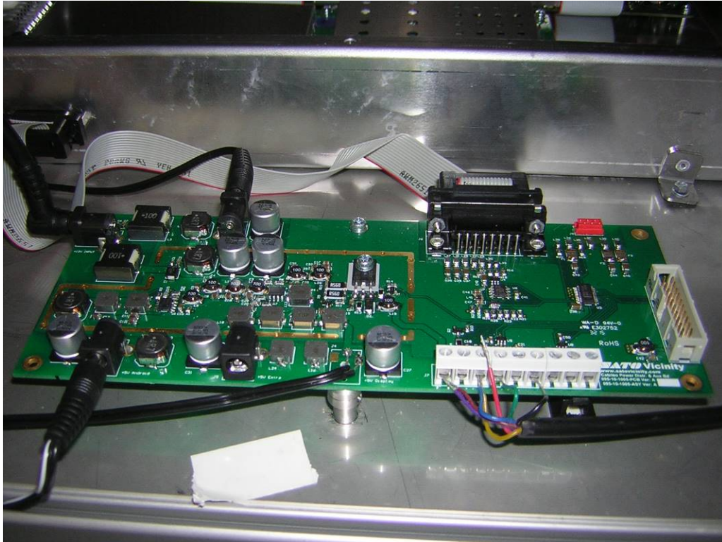
PCB Cabinet Power
