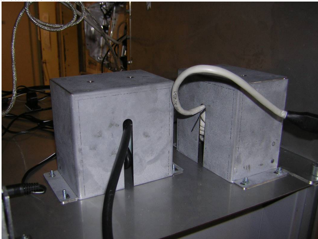
Ferrite locations on cables
