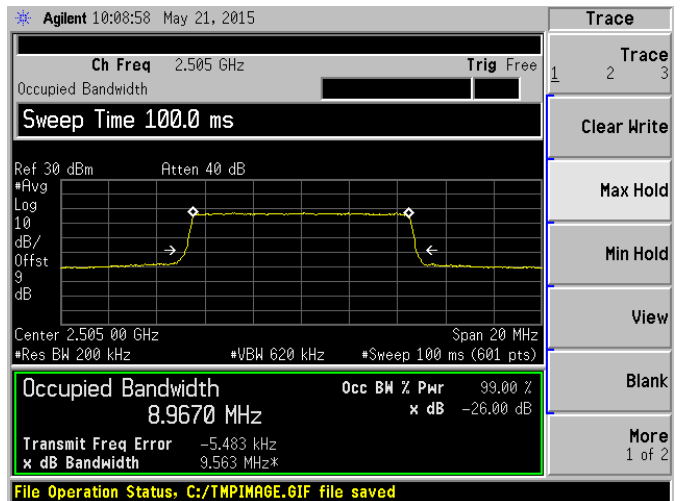
Band 7 QPSK 10 MHz Bandwidth RB6#0 LCH
