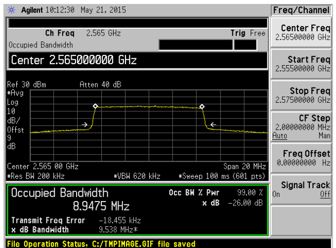
Band 7 QPSK 10 MHz Bandwidth RB6#0 HCH
