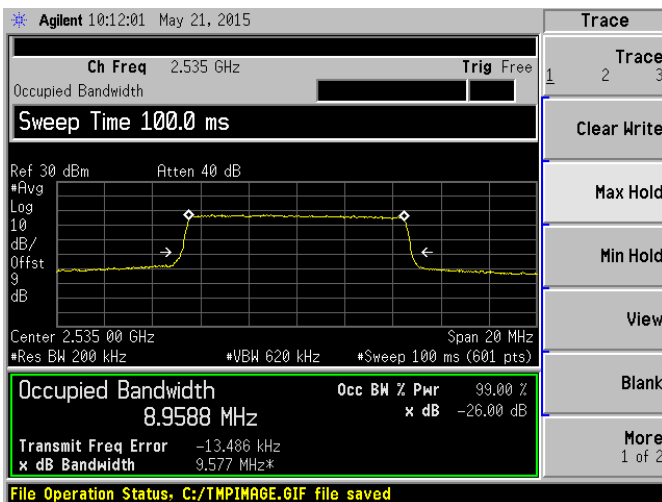
Band 7 QPSK 10 MHz Bandwidth RB6#0 MCH
