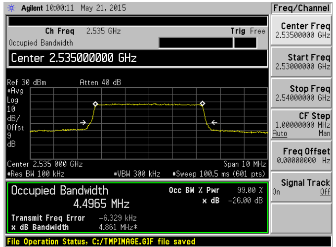
Band 7 QPSK 5 MHz Bandwidth RB6#0 MCH
