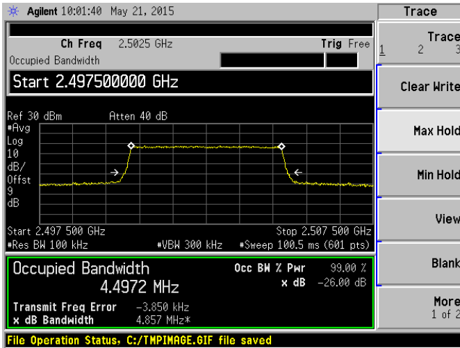
Band 7 QPSK 5 MHz Bandwidth RB6#0 LCH
