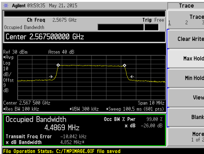
Band 7 QPSK 5 MHz Bandwidth RB6#0 HCH
