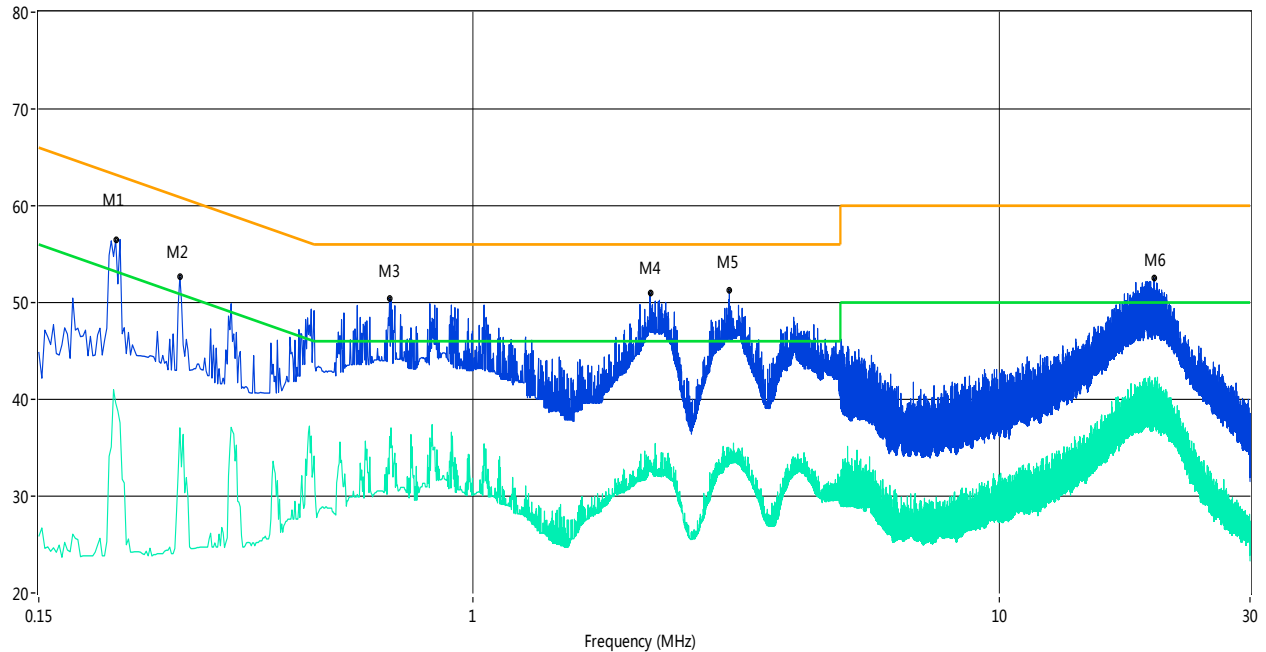
PHASE L
