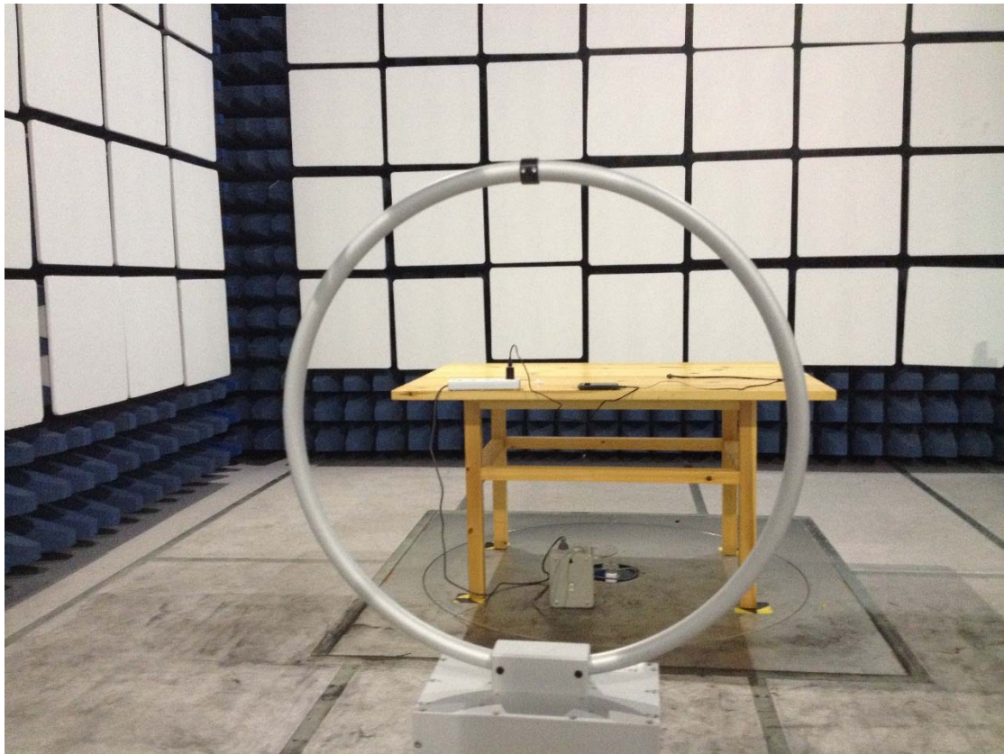
Below 30MHz (Camera Test Mode)
