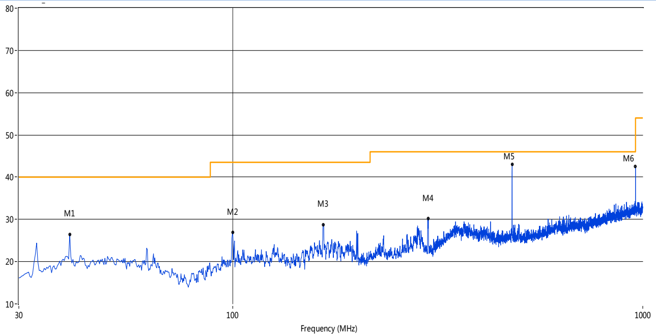
GFSK LOW CHANNEL 30MHz to 1GHz, ANT V
