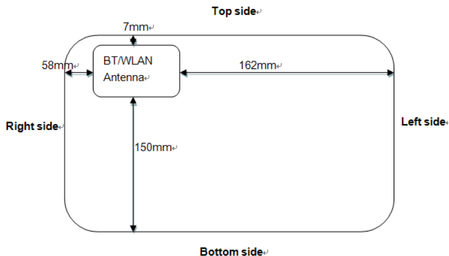
Figure 2: The antenna positions of the DUT
