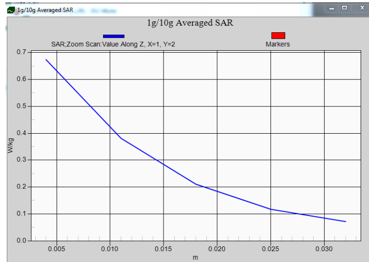
Plot 1: Rear Side (WLAN2450-Middle Channel-Channel 6-2437MHz(1Mbps))
