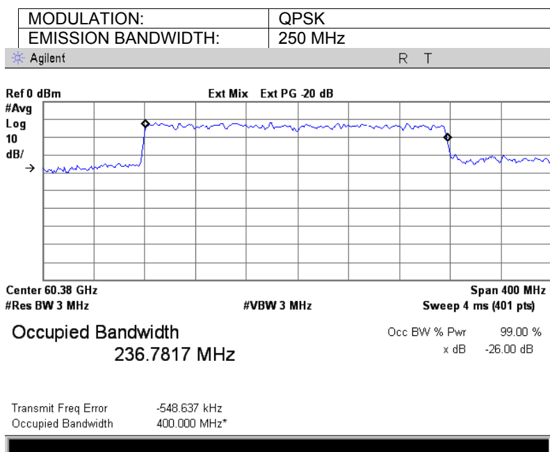
Plot 7.2.8 Occupied bandwidth at the mid frequency
