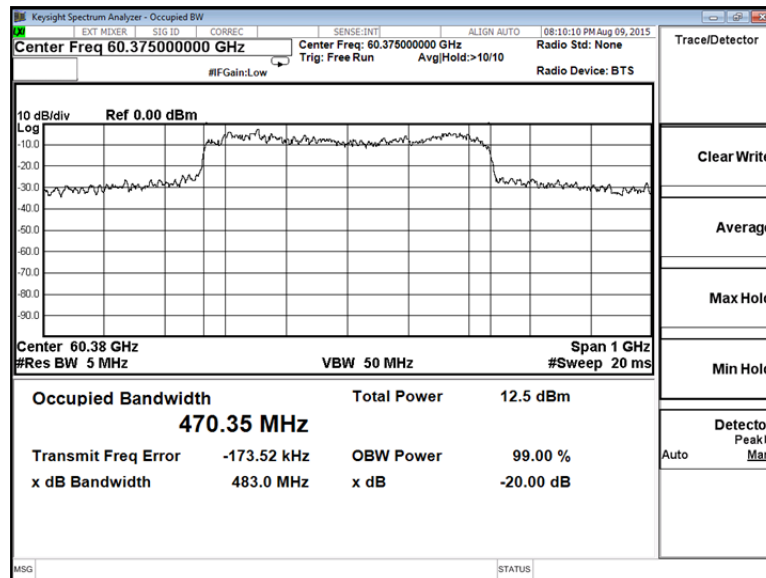
Plot 7.2.12 Occupied bandwidth at the high frequency
