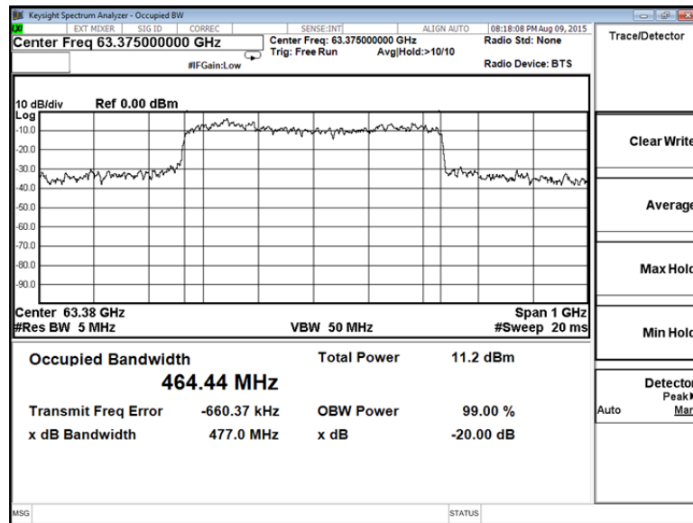
Plot 7.2.10 Occupied bandwidth at the low frequency
