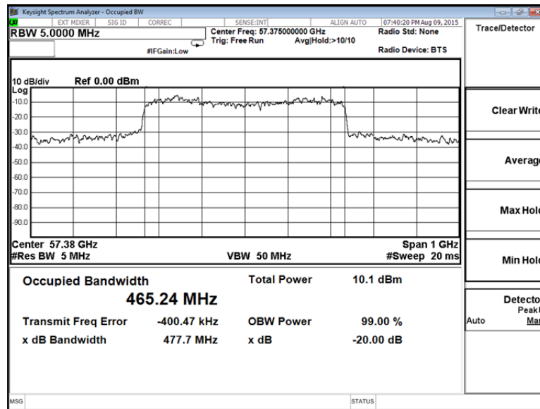
Plot 7.2.8 Occupied bandwidth at the mid frequency
