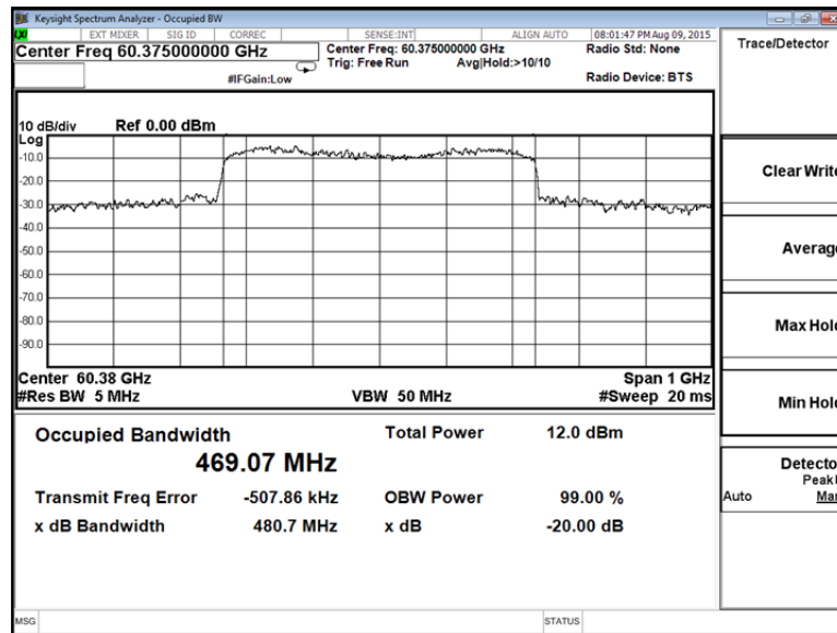
Plot 7.2.6 Occupied bandwidth at the high frequency
