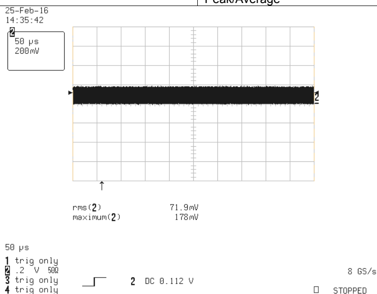
Plot 7.1.4 Output power test result at the low frequency
