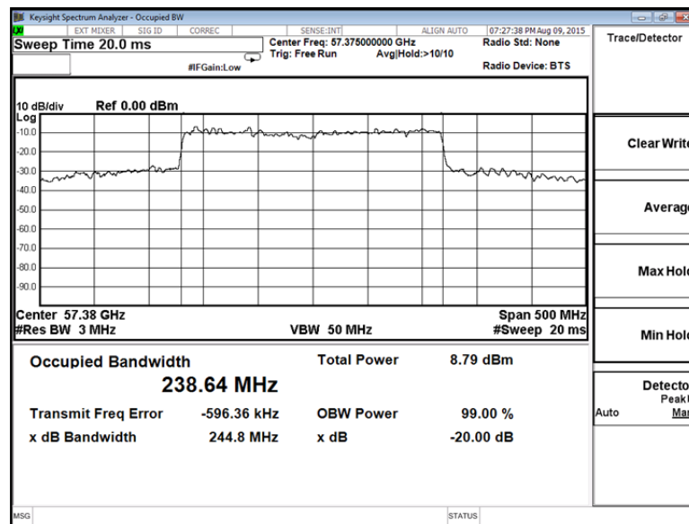
Plot 7.2.2 Occupied bandwidth at the mid frequency
