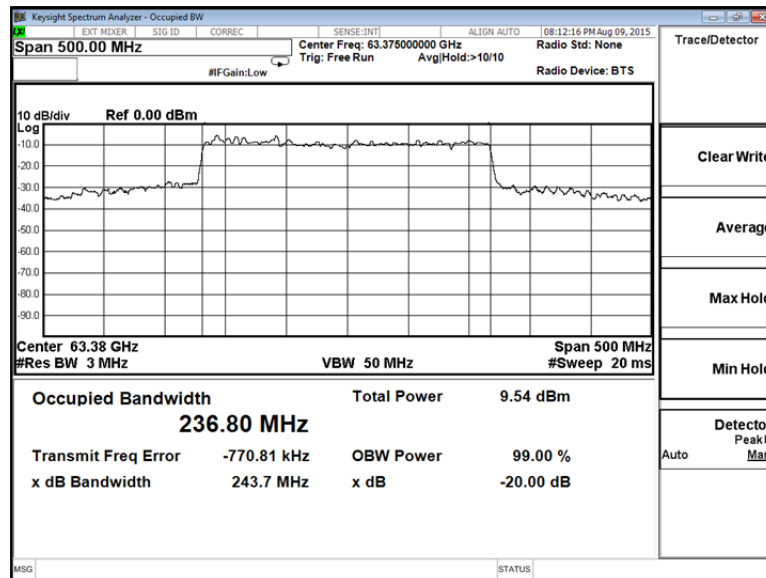
Plot 7.2.4 Occupied bandwidth at the low frequency
