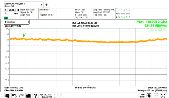
Plot 7.4.54 Spurious emission measurements in 180 - 190 GHz range
