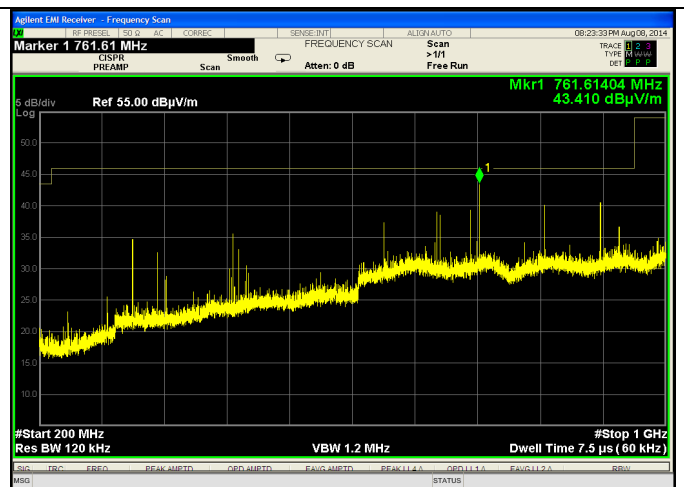
200-1000 MHz Horizontal
