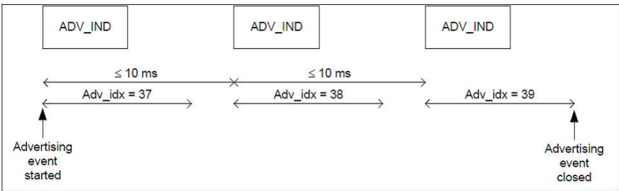
Figure F2: Connectable undirected advertising event with only advertising PDUs
