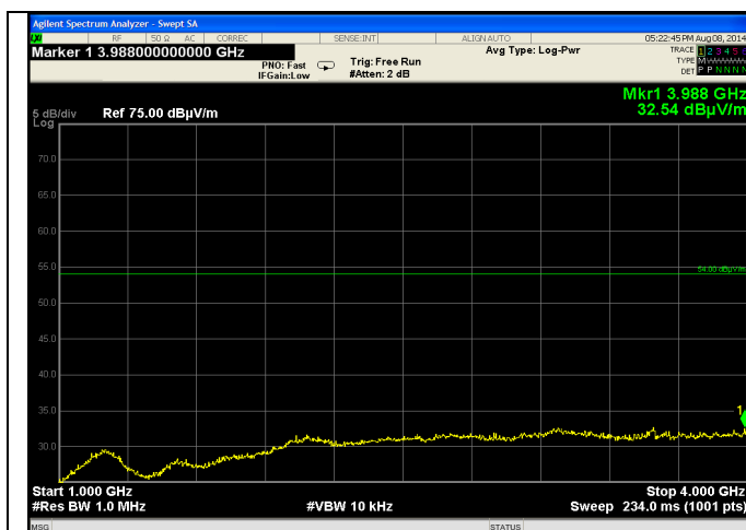
1-4 GHz (Reduced VBW)
