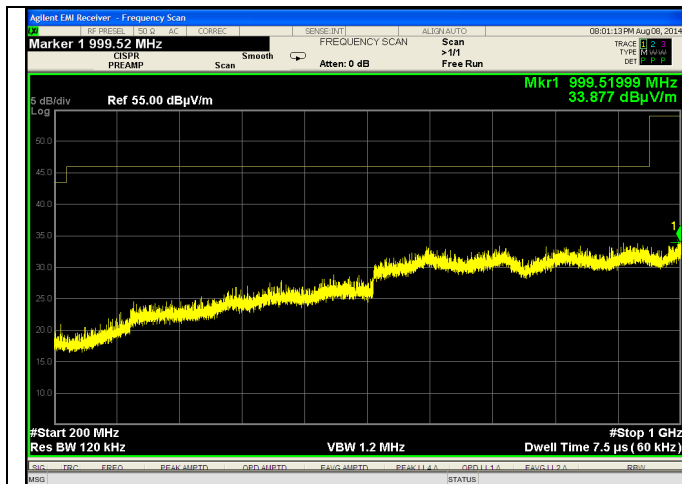
200-1000 MHz Vertical
