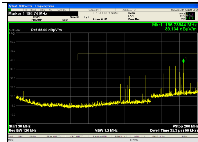
30-200 MHz Vertical
