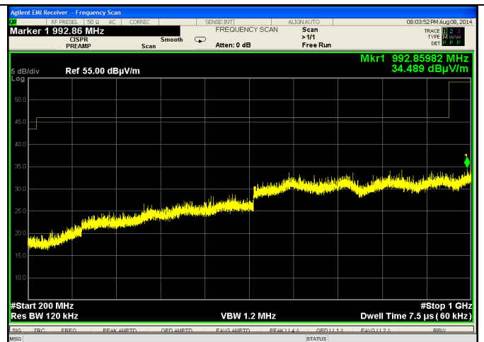
200-1000 MHz Horizontal
