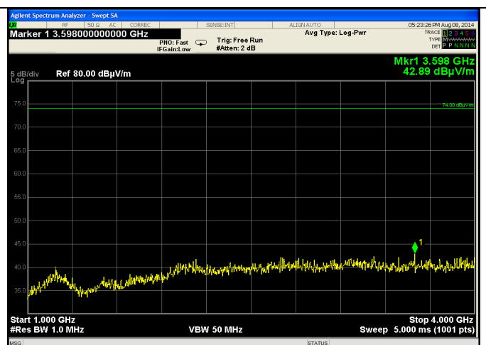
1-4 GHz (Peak)
