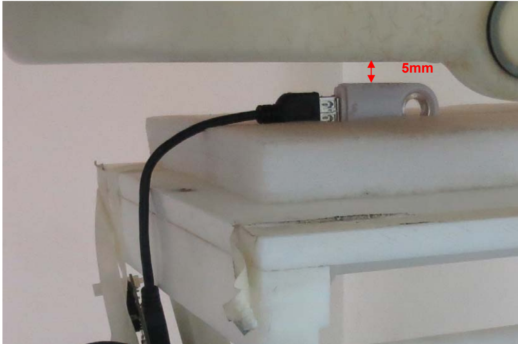
Picture 6: Right Edge, the distance from EUT to the bottom of the Phantom is 5mm
