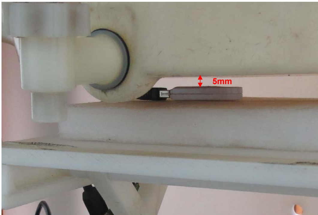
Picture 5: Left Edge, the distance from EUT to the bottom of the Phantom is 5mm
