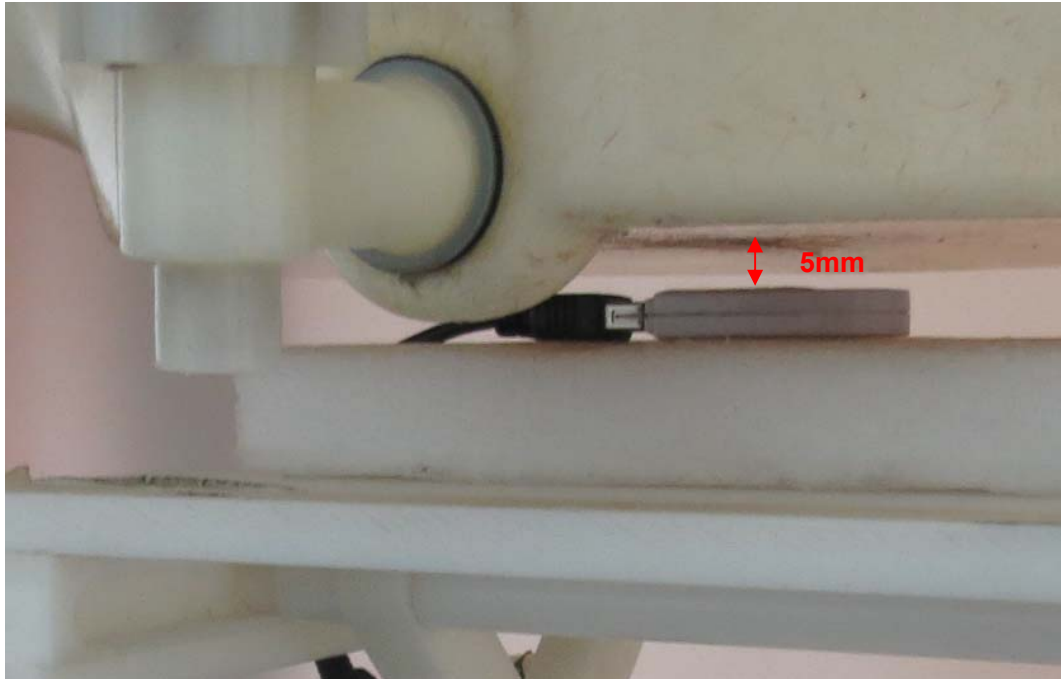
Picture 4: Back Side, the distance from EUT to the bottom of the Phantom is 5mm
