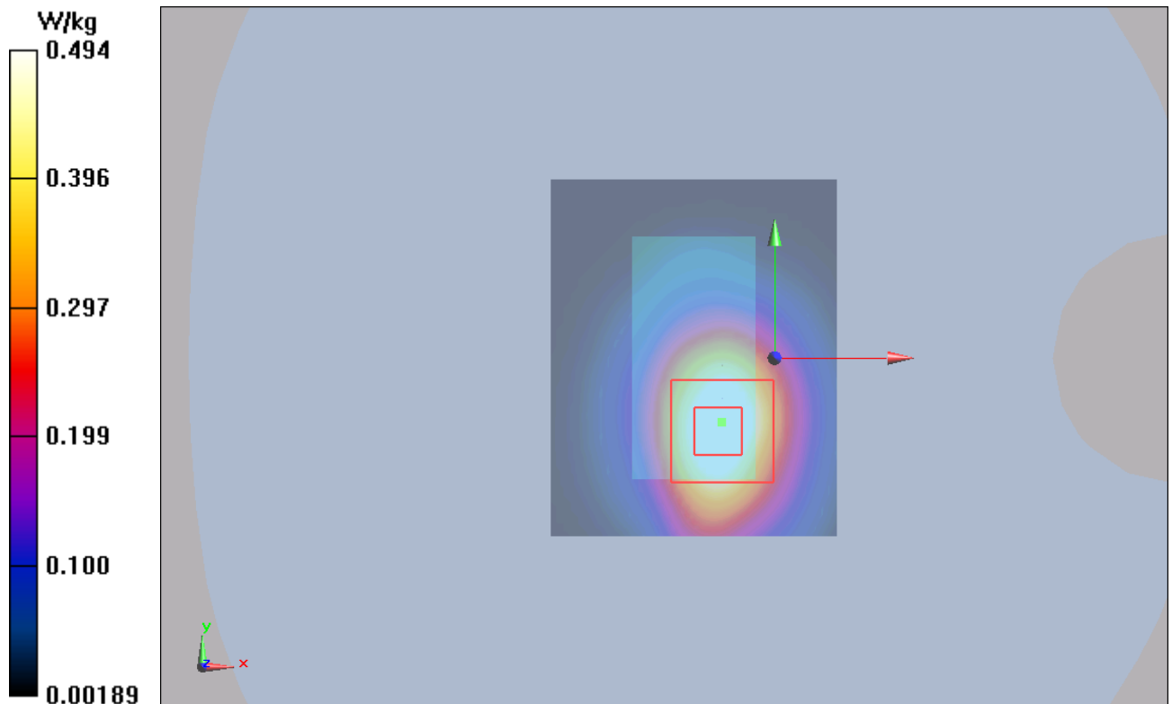
Figure 7 Back Side High 802.11b Channel 11
