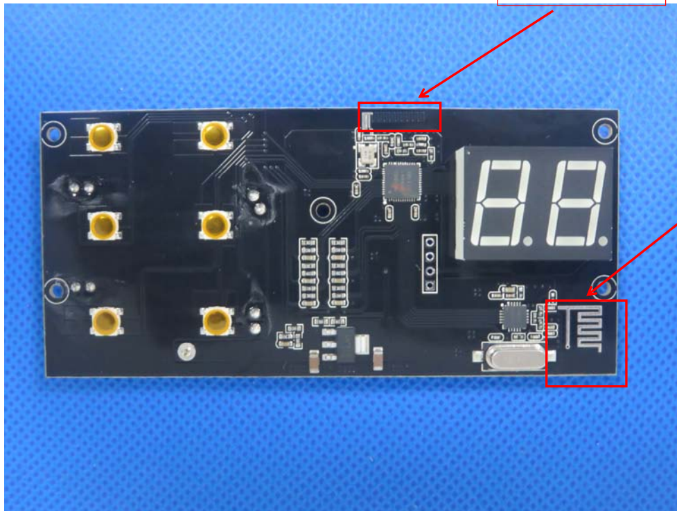
BT4.0 Antenna
