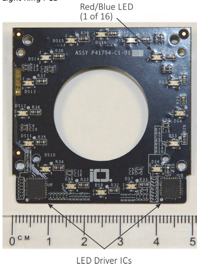
Figure 5: Light ring PCB. No active components on side B
