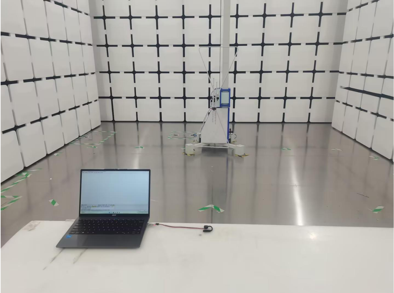
Radiated Spurious Emission Test View -Left earphone
