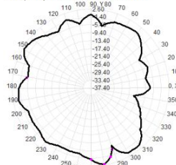
Total(H-XY), Max= 1.92dBi, CirD=17.25
