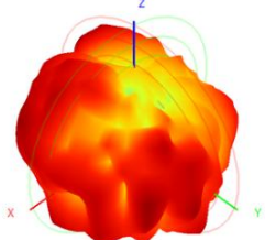
6400.0MHz H+V. Eff. 42.2%
