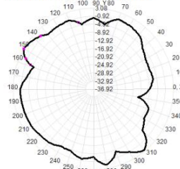
Total(H-XY), Max= 3.08dBi, CirD=17.80
