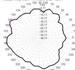
Total(H-XY), Max= 1.76dBi, CirD=12.84
