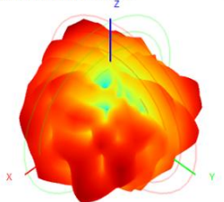
7000.0MHz H+V, Eff. 44.9%
