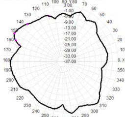
Total(H-XY), Max= 3.00dBi, CirD=11.91
