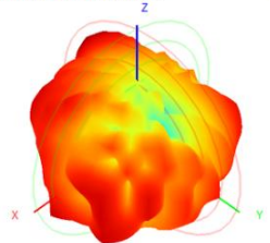
6800.0MHz H+V, Eff. 42.8%
