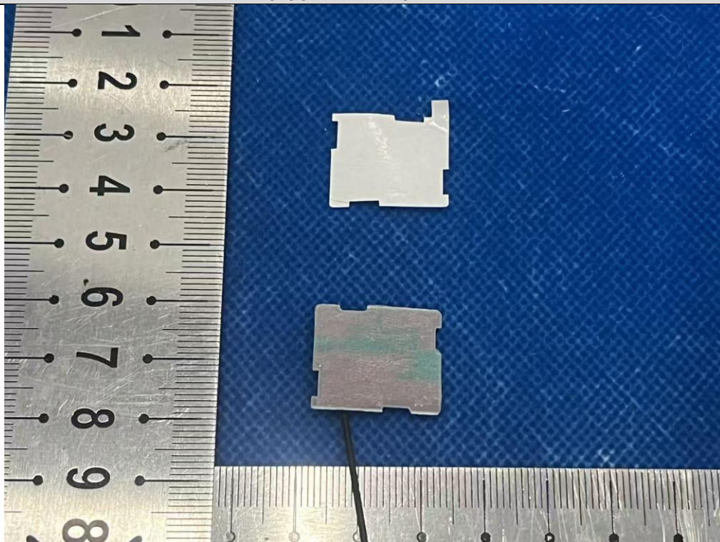
WiFi 7 Chip (QCC2027PB) Antenna Photo
