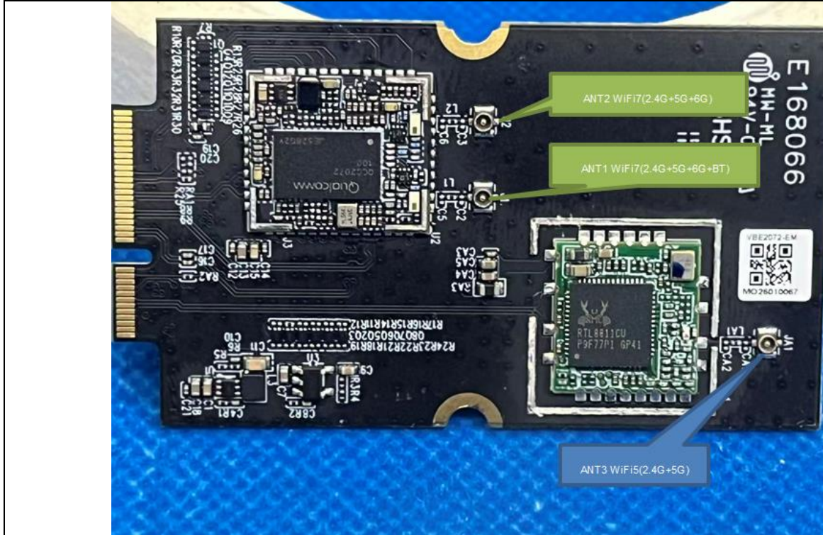
Antenna Ports Photo
