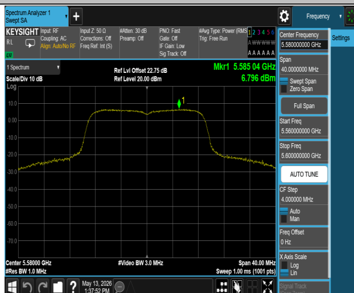
11N20SISO_Ant3_5580
