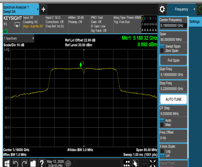
11N40SISO_Ant3_5190
