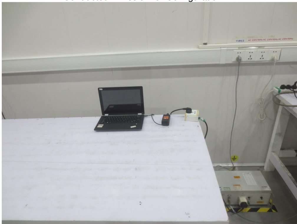
Conducted Emission for Configuration: 2#
