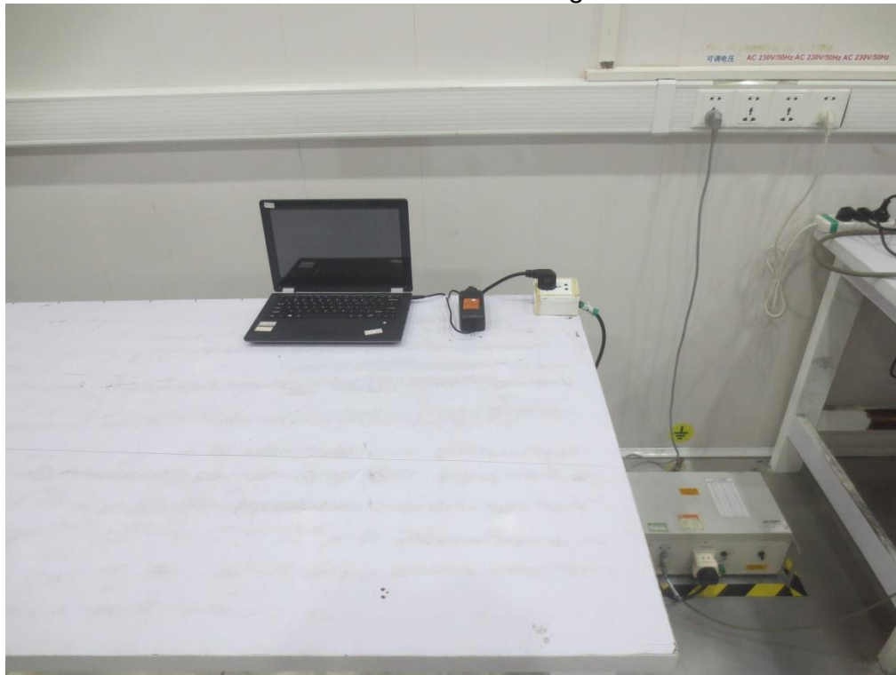
Conducted Emission for Configuration: 1#
