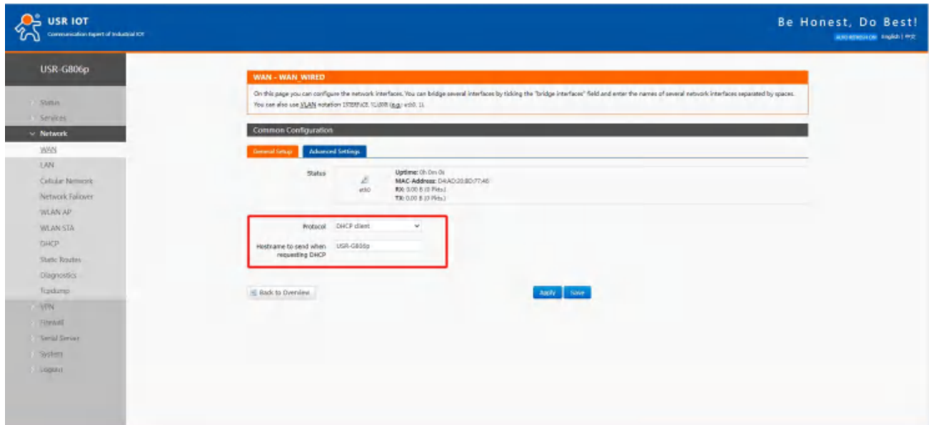
Pic 16 WAN
