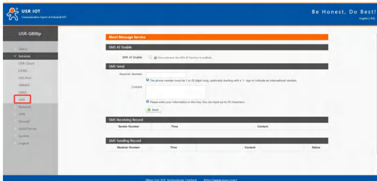
Pic 75 SMS
