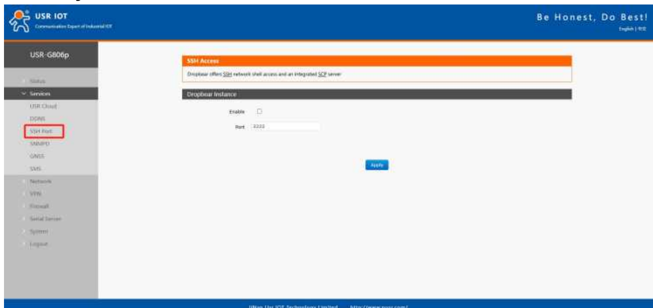
Pic 74 SSH
