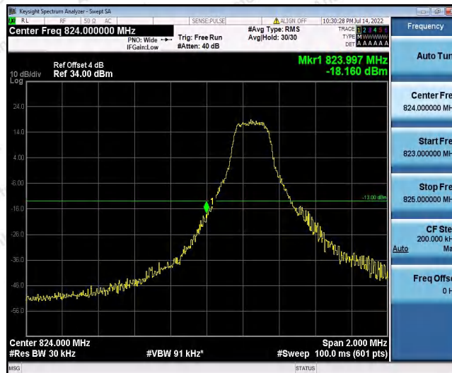
Band5-1.4MHz-QPSK-20407-1RB#5
