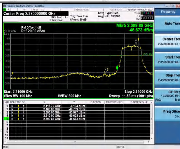
11G_Ant2_Low_2412
