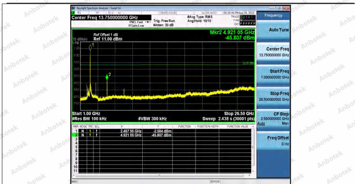
11N20SISO_Ant2_2462_0~Reference
