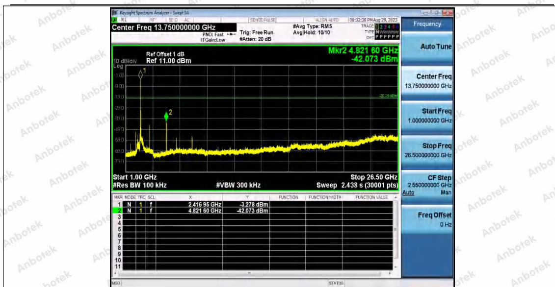
11N20SISO_Ant2_2412_0~Reference
