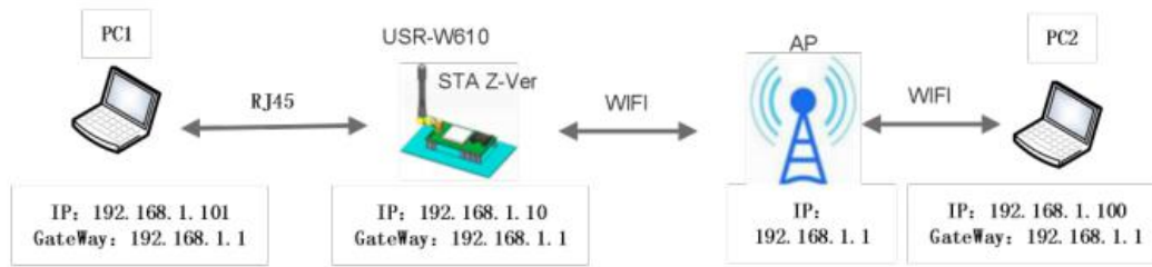
Figure 12 Bridge mode
