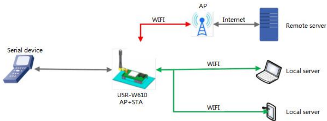
Figure 7 AP+STA mode
