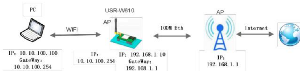
Figure 10 AP+WAN application
