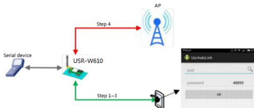
Figure 20 Usrlink
