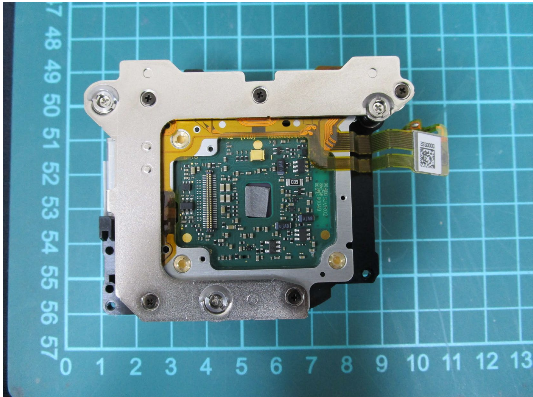
(11) EUT Photo
