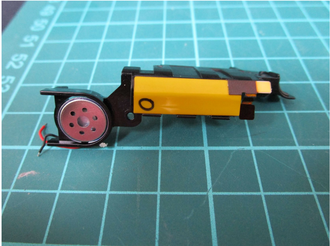
(23) EUT Photo
