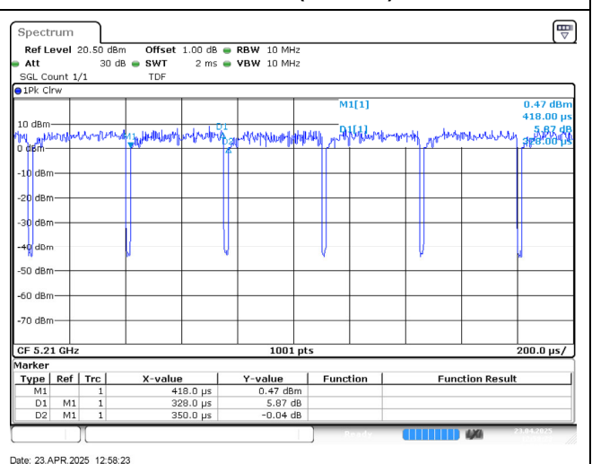
802.11ac (80 MHz)
