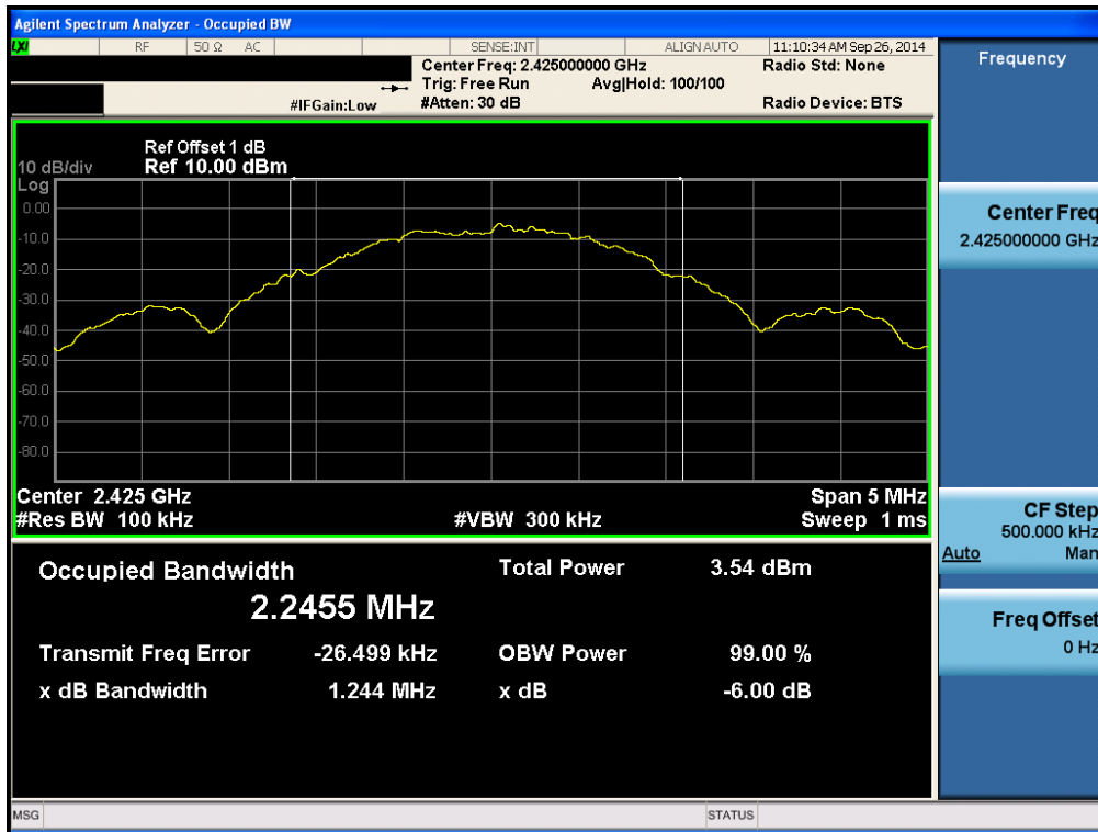
6 dB Bandwidth
