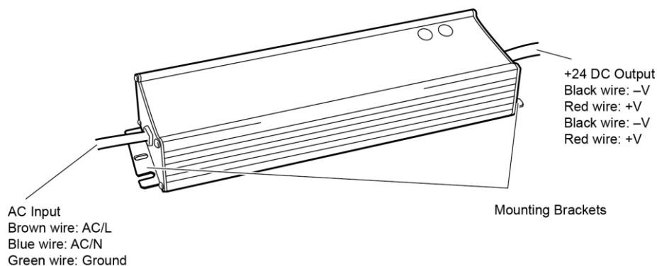
Figure 8. Deployment Kit Power Supply
