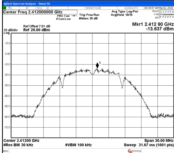
802.11b Chain 0-Low channel
