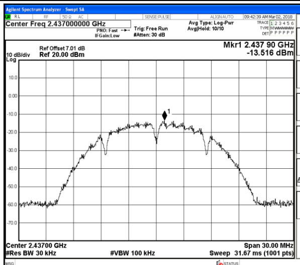
802.11b Chain 0-Middle channel
