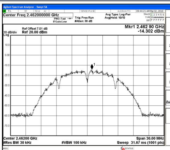
802.11b Chain 0-High channel
