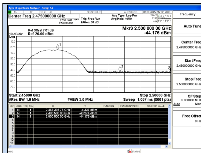
Channel 11 / 2462 MHz – Peak
