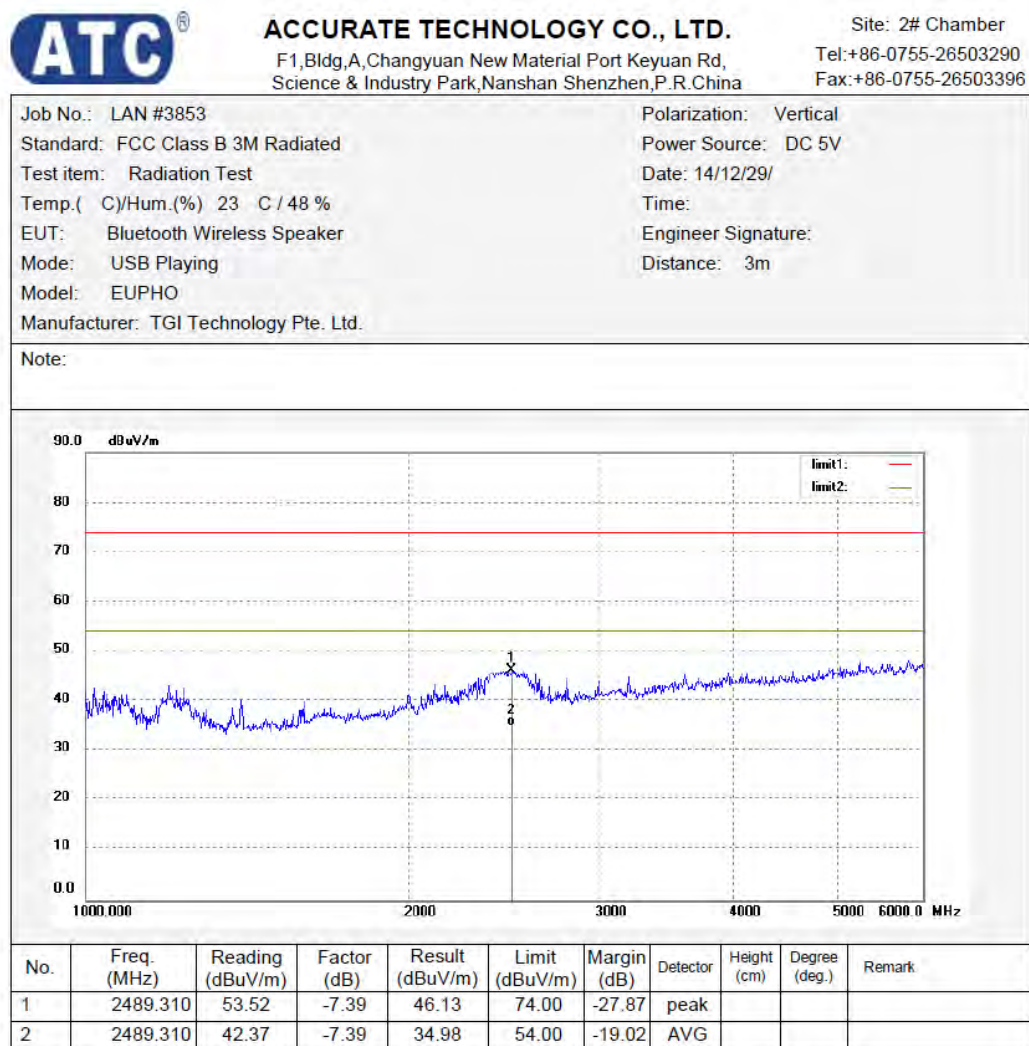
Figure 66: Test figure of Radiated emissions, Mode D, Above 1GHz, Vertical
