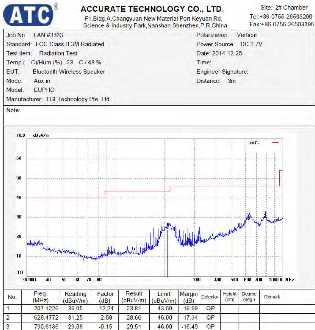
Figure 60: Test figure of Radiated emissions, Mode C, Below 1GHz, Vertical
