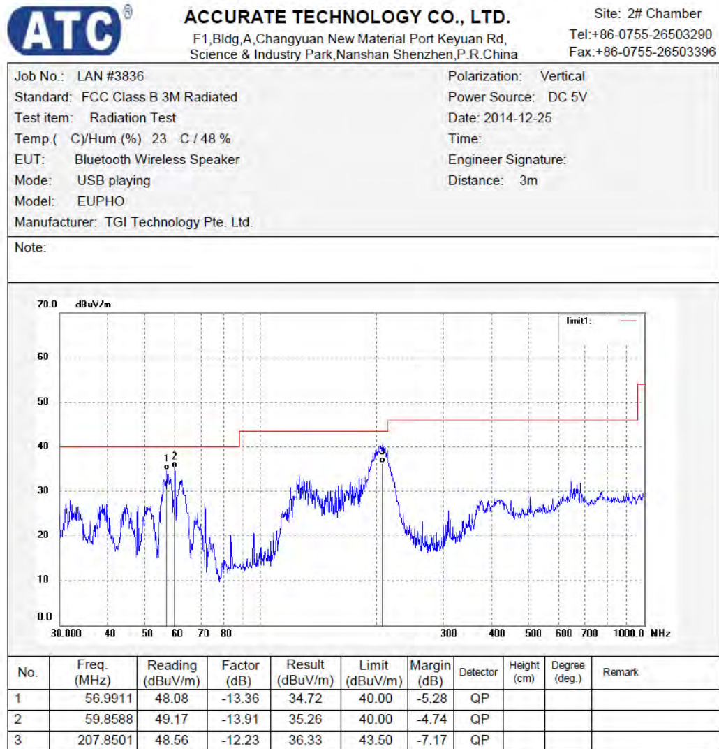
Figure 64: Test figure of Radiated emissions, Mode D, Below 1GHz, Vertical
