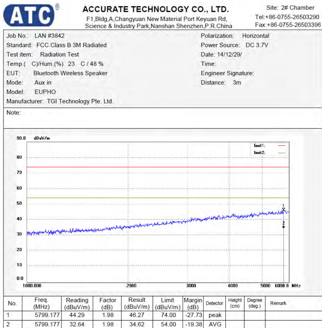
Figure 61: Test figure of Radiated emissions, Mode C, Above 1GHz, Horizontal
