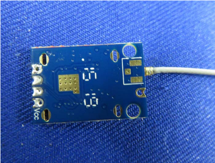
Figure 24 PCB of the EUT-BackView
