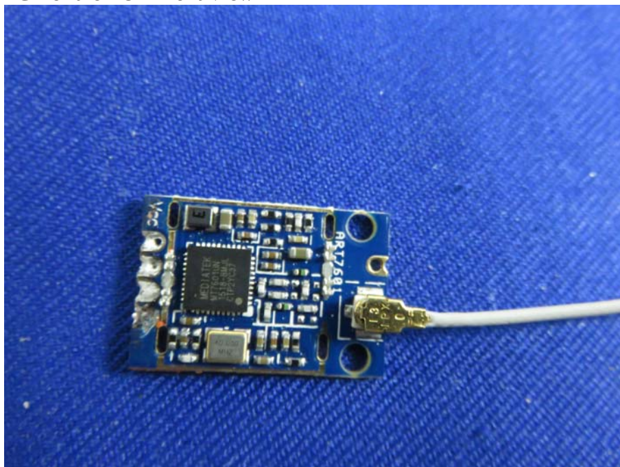
Figure 23 PCB of the EUT-Front View
