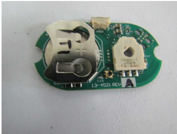
Figure 1: PCB Top
