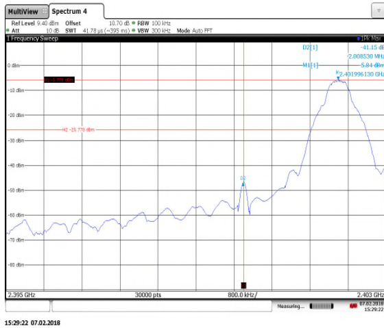
Figure 7.5.1.2-4: Lower Band-edge – LCH
