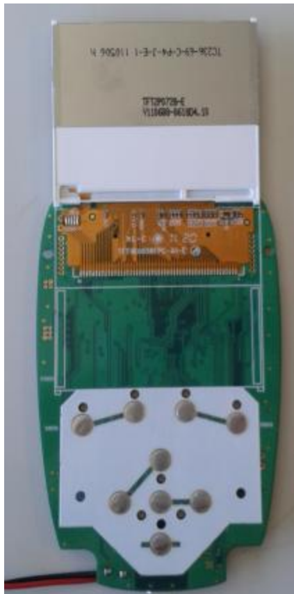
Top side of PCB to show what's underneath the display and keypad, including bottom side of display and keypad
