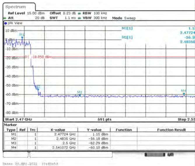
3DH5(2480)-Hopping on
