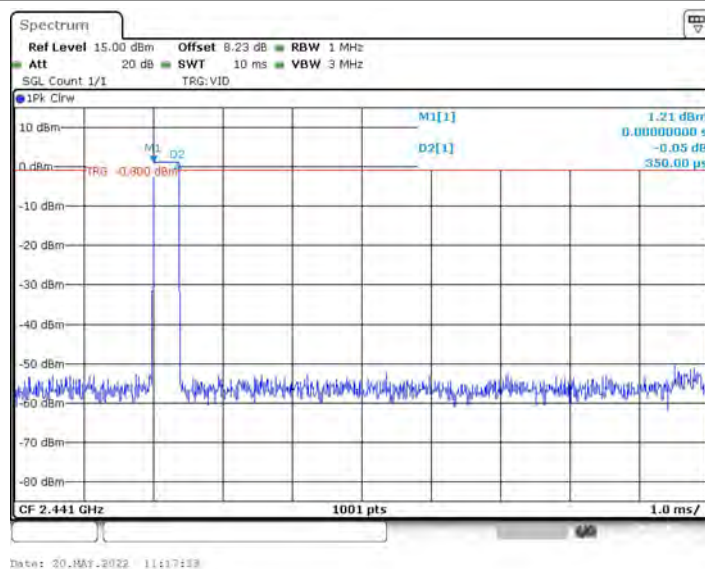
GFSK mode-DH1
