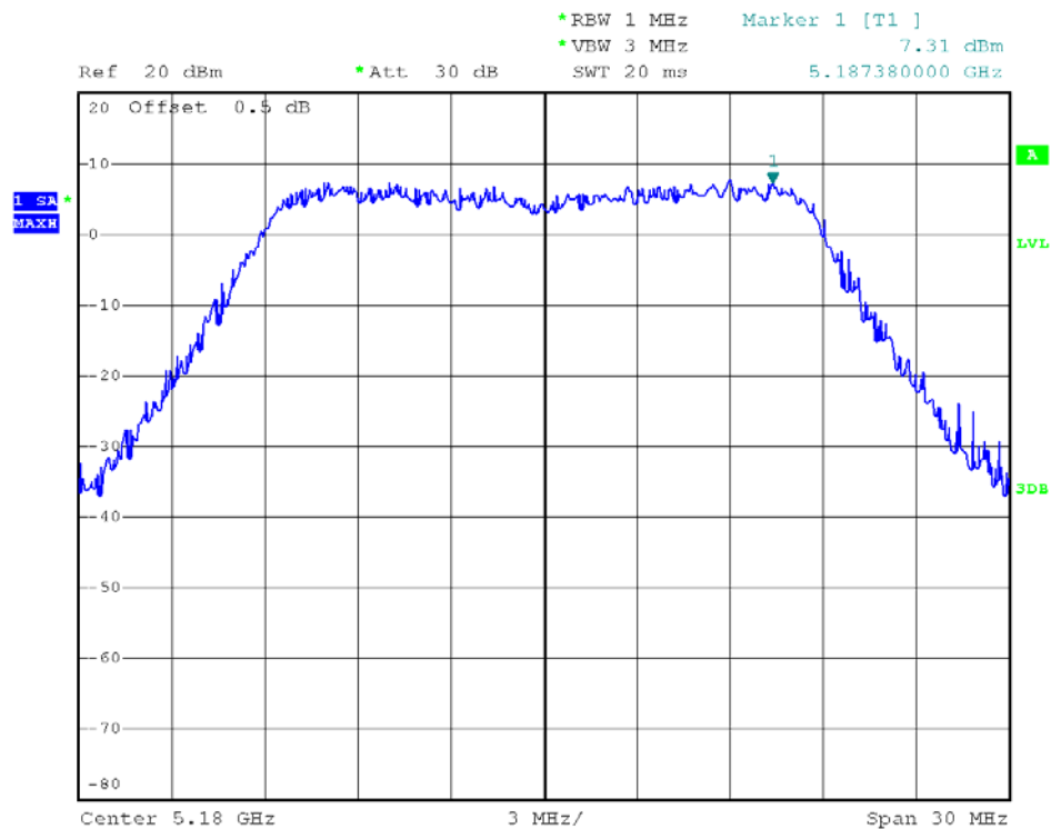
Antenna A - 802.11a – 5180MHz
