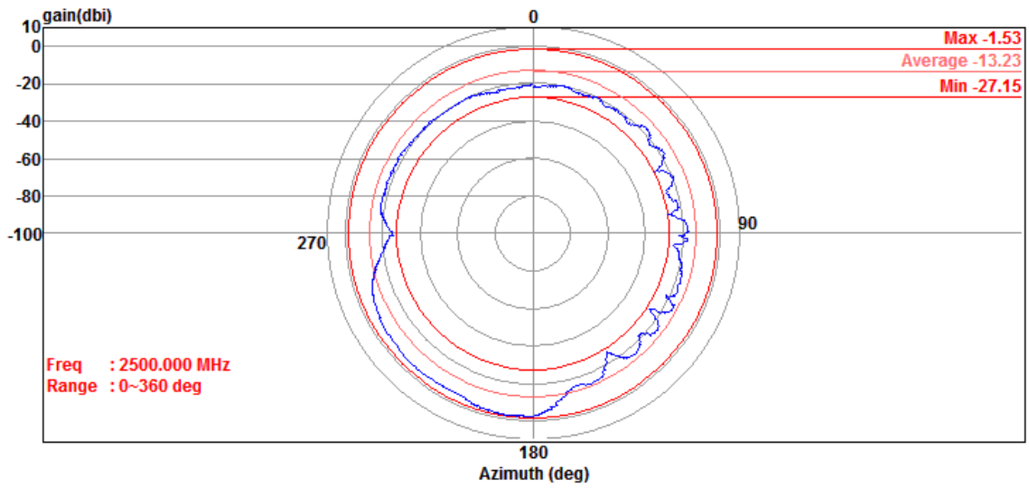
Figure 5: 2500MHz Vertical
