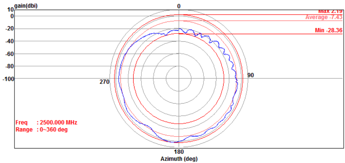
Figure 6: 2500MHz Horizontal
