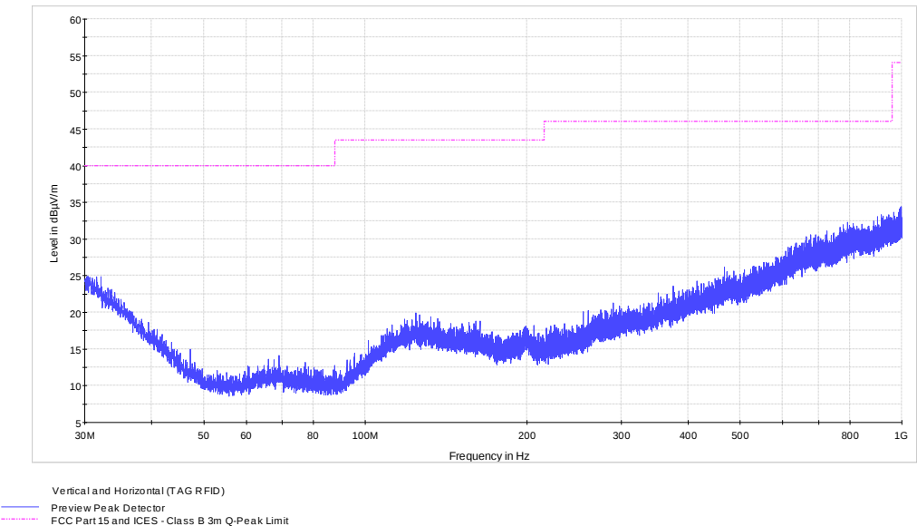
Figure 8.3-1: Spurious emissions below 1 GHz (Channel 10)
