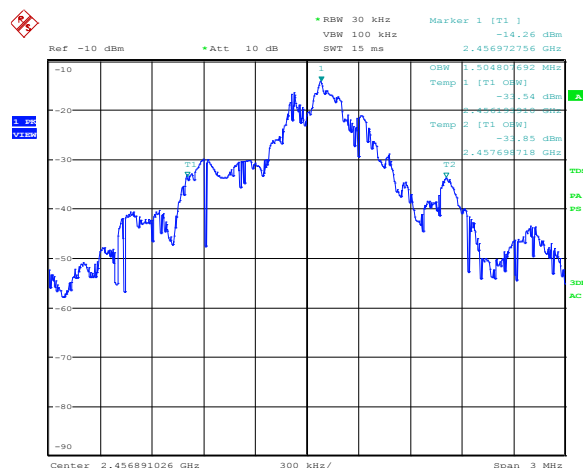
Figure 8.1-4: 99% occupied bandwidth (Channel 57)
