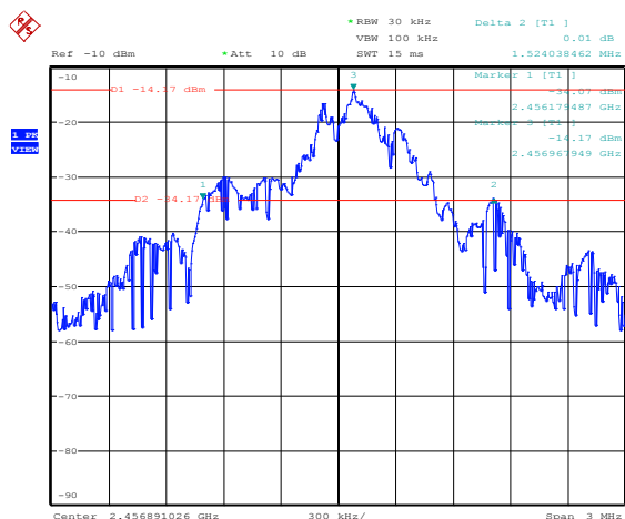
Figure 8.1-3: 20 dB bandwidth (Channel 57)
