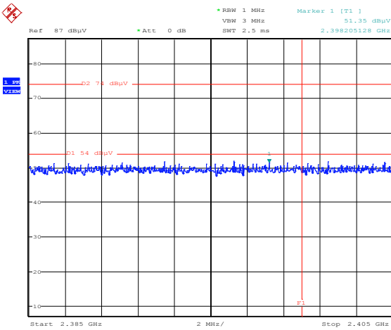
Figure 8.3-7: Lower band edge emission at 2400 MHz (Tx set to Channel 10) F1= 2400 MHz
