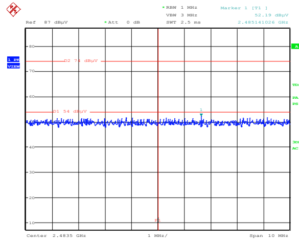
Figure 8.3-8: Upper band edge emission at 2483.5 MHz (Tx set to Channel 57) F1 = 2483.5 MHz
