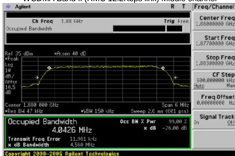
WCDMA Band II (RMC 12.2Kbps link) Middle channel
