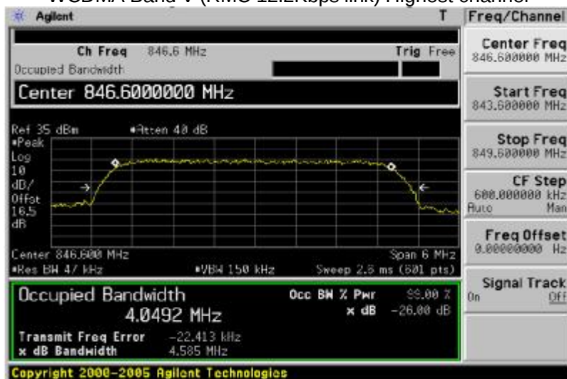
WCDMA Band V (RMC 12.2Kbps link) Highest channel
