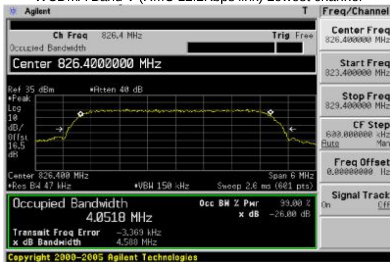
WCDMA Band V (RMC 12.2Kbps link) Lowest channel
