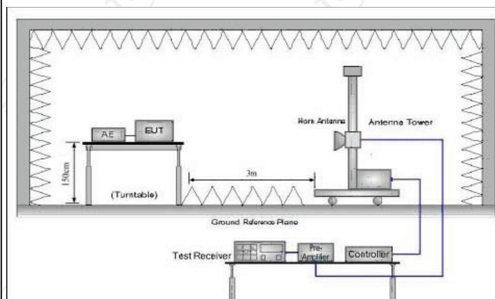
Above 1GHz
