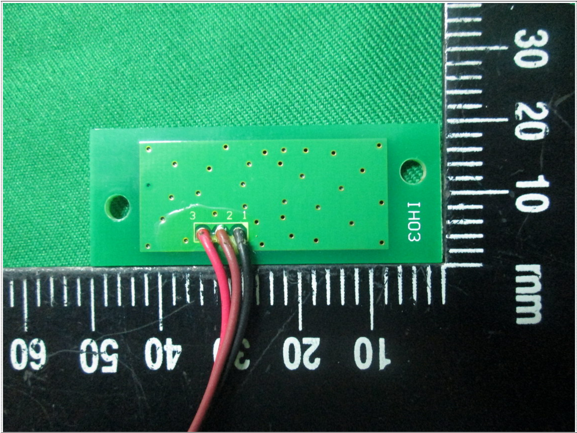
Rear View of Controller Board
