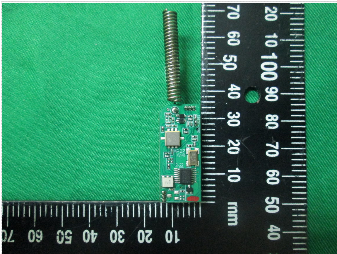
Front View of Module Board
