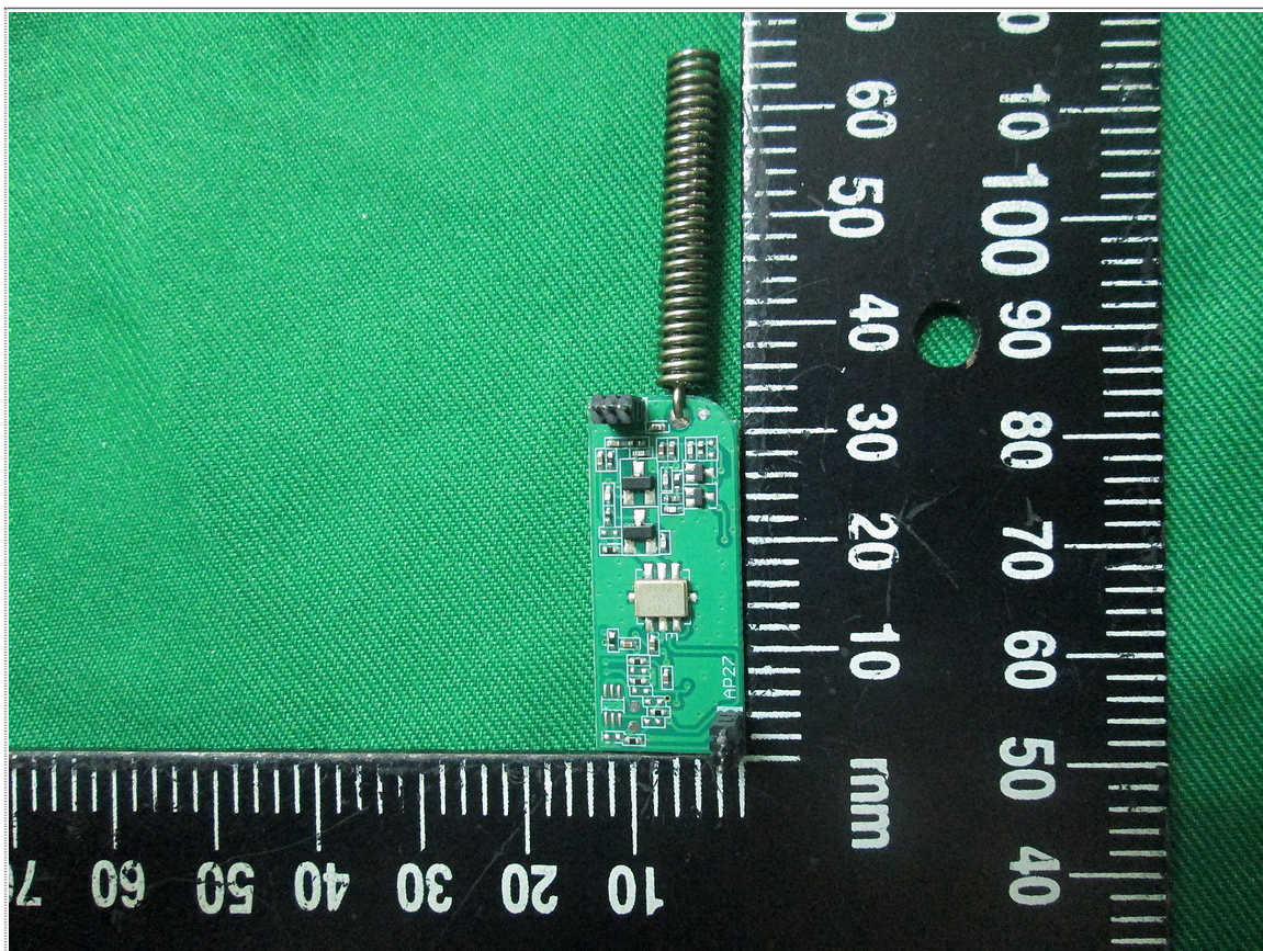
Rear View of Module Board
